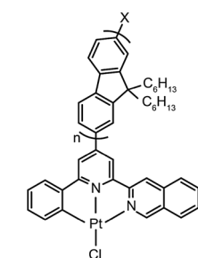
172: n = 1 , X = \text{H}
