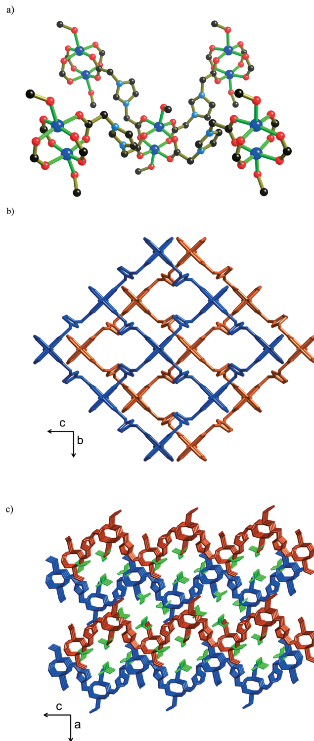
Fig. 1 The structure of [\text{Cu}_2(\text{imdc})_2(\text{CH}_3\text{OH})_2](\text{BF}_4)_2 \cdot \text{solvent} ( 1 ) showing: a) part of the undulating [\text{Cu}_2(\text{imdc})_2(\text{CH}_3\text{OH})_2]^{2+} square grid sheet in which \text{Cu}_2 units are bridged by \text{imdc}^- anions; coordinate bonds are indicated by green connections, atom colour code: Cu – deep blue, O – red, N – light blue, C – black b) a stick representation indicating the relative arrangement of the 2D networks viewed along the stacking direction (along the a axis); the methyl groups of the methanol have been omitted for clarity c) a view almost normal to the stacking direction showing the channels between the sheets that run parallel to the b axis; the \text{BF}_4^- anions are indicated in green. Non-coordinated solvent molecules and hydrogen atoms have been omitted for clarity.
