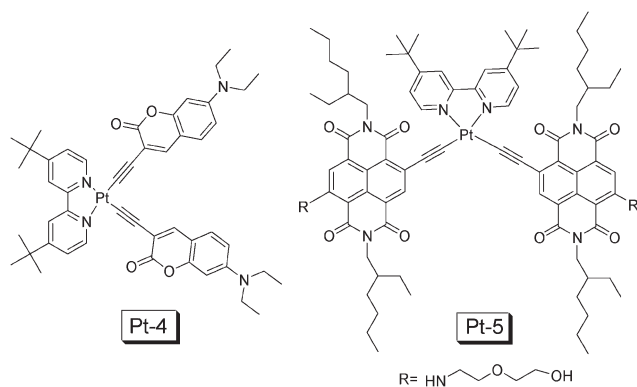
Fig. 14 N^N Pt(II) complexes Pt-4 and Pt-5 that show intense absorption of visible light used as triplet sensitizers for TTA upconversion. The compounds Pt-4 and Pt-5 are from ref. 36 and 37, respectively.
