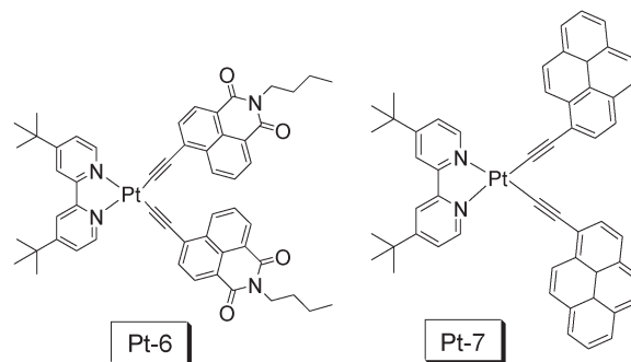
Fig. 15 N^N Pt(II) bisacetylide complexes that show prolonged T_1 excited state lifetimes ( \tau = 124.0 \mu\text{s} for Pt-6 and \tau = 73.6 \mu\text{s} for Pt-7 ) used as triplet sensitizers for TTA upconversion. The compounds are from ref. 18 and 39, respectively.
