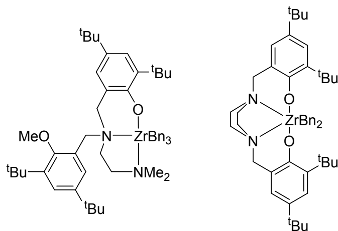
Figure 4. Further examples of light-enhanced hydrophosphination via zirconium compounds that were originally reported by Yuan and Yao. 93
