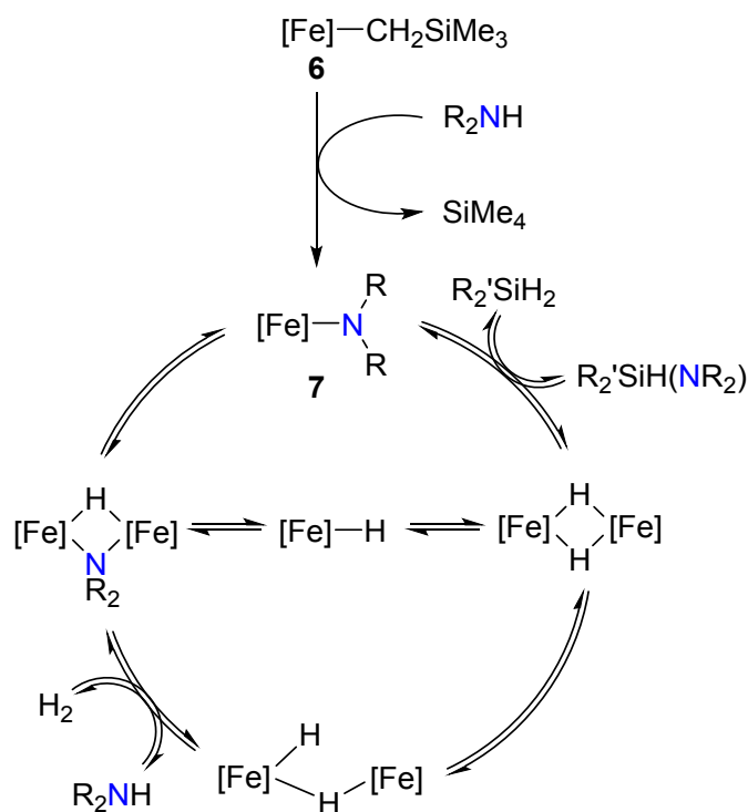
Scheme 6. Mechanism for Si–N heterodehydrocoupling catalysed by iron \beta -diketiminato. 26
