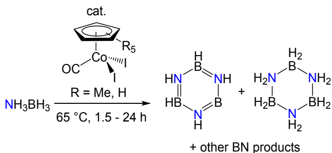
Scheme 10. Amine–borane dehydrocoupling catalysed by a piano-stool cobalt compound to afford saturated and unsaturated products. 47
