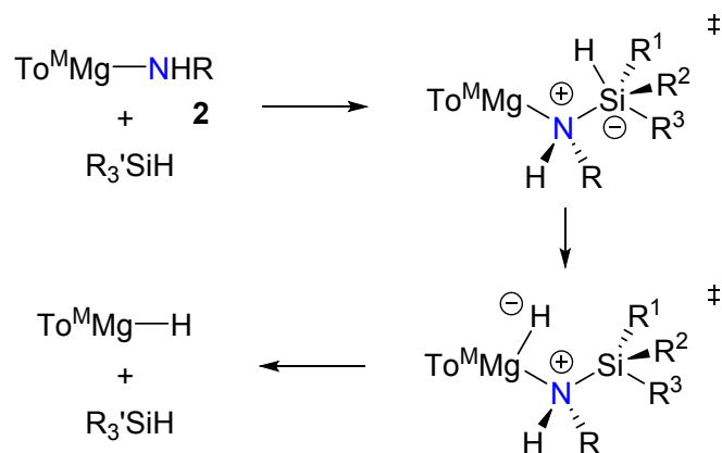
Scheme 4. Nucleophilic attack on silane by (\text{To}^{\text{M}})\text{MgNR}_2 . 19
