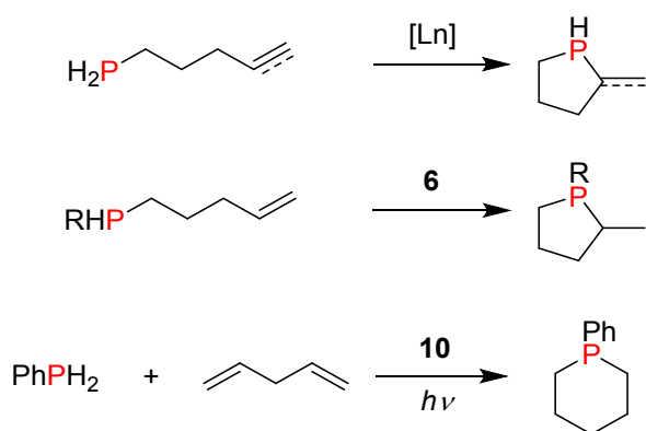
Scheme 20. Synthesis of five- and six-membered phosphine products via metal-catalysed hydrophosphination. [Ln] = Cp* 2 LnCH(SiMe 3 ) 2 . 74, 86, 87
