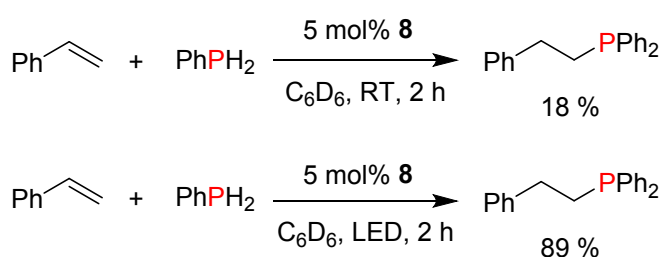
Scheme 21. Visible-light-enhanced hydrophosphination of alkenes with PhPH 2 . 86
