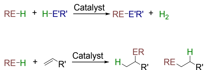
Scheme 1. General reactions for catalytic dehydrocoupling (top) and hydrofunctionalization (bottom).
