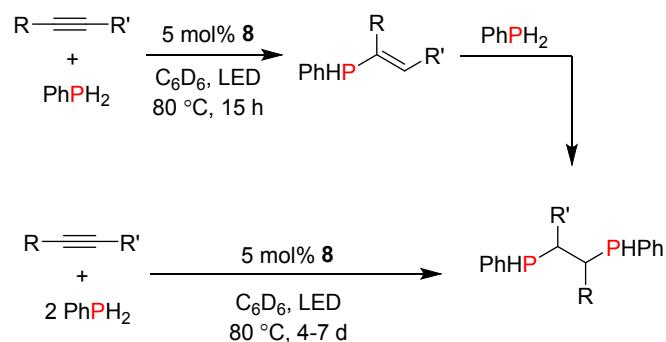
Scheme 19. Zirconium-catalysed double hydrophosphination of internal alkynes using \text{PhPH}_2 . 6
