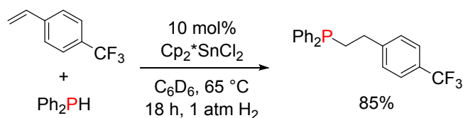
Scheme 13. Hydrophosphination of p -substituted styrene substrates with \text{Ph}_2\text{PH} mediated by \text{Sn}(\text{IV}) catalyst. 54
