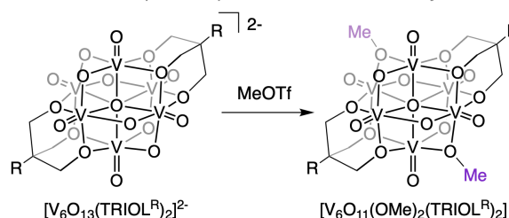
Figure 1. Schematic representation of surface functionalisation of metal oxide nanomaterials (top); here, we present the sequential alkylation of high-valent POV-alkoxide clusters as homogeneous model complexes for the physicochemical implications of organofunctionalisation of metal oxide surfaces.
