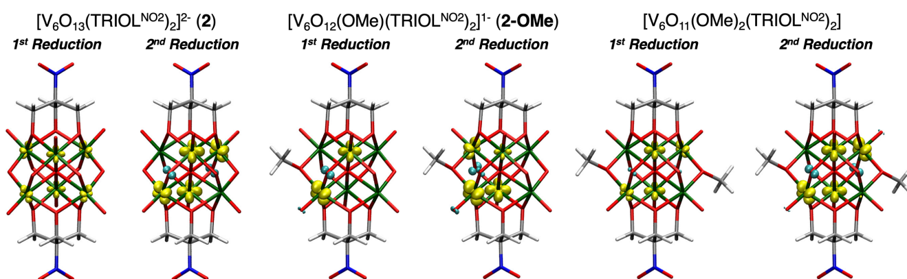
Figure 7. Spin density of reduced 2 , 2-OMe , and para -[V 6 O 11 (OMe) 2 (TRIOl NO2 ) 2 ] at M06/def2-TZVP//M06-L/def2-TZVP,def2-SVP level of theory. Vanadium in dark green, oxygen in red, nitrogen in blue, carbon in grey, and hydrogen in white. Alpha spin density in yellow and beta spin density in cyan. Isosurface = 0.4. Additional spin density plots for reduced variants of 1-OMe and meta - 1-(OMe) 2 can be found in Figure S17.
