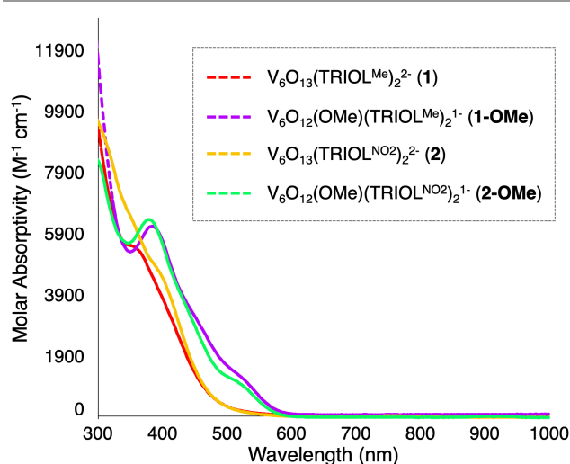
Figure 5. Electronic absorption spectra of complexes 1 , 1-OMe , 2 , and 2-OMe collected in MeCN at 21 °C.
