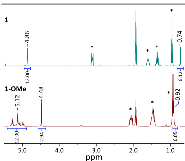
Figure 2. 1 H NMR spectra of complexes 1 (top, blue) and 1-OMe (bottom, red) collected in CD_3CN at 21 °C. Formation of the alkylated species 1-OMe is indicated by the appearance of a singlet peak belonging to the bridging methoxide ligand at 4.48 ppm, along with a downfield shift of the signal corresponding to the terminal methyl group of the capping triol ligand (0.74 and 0.92 ppm for 1 and 1-OMe respectively). Additionally, the singlet peak corresponding to the methylene group of the parent cluster 1 (4.86 ppm) splits into a multi-peak pattern upon formation of the alkylated species 1-OMe (peaks centred at 5.12 ppm). Peaks labelled with * indicate signals belonging to the cations [tBu_4N]^+ and [tBu_4P]^+ for 1 and 1-OMe respectively. Peak assignments for alkylated species can be found in figures S1 and S7 for 1-OMe and 2-OMe respectively.
