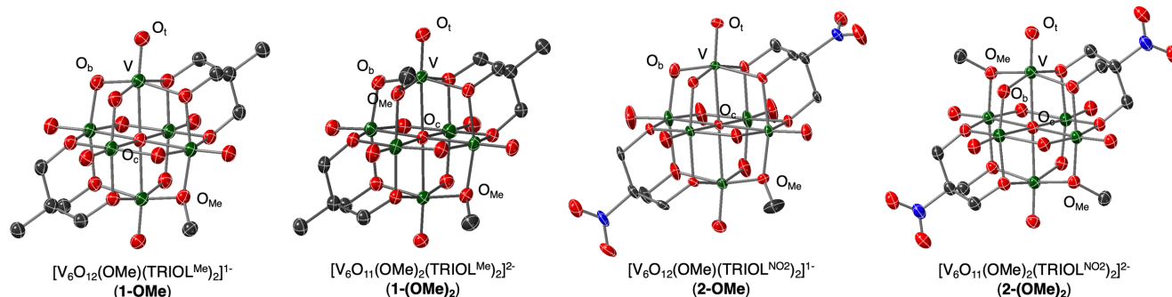
Figure 3. Molecular structures of [V_6O_{12}(OMe)(TRIOlMe)_2]^{1-} ( 1-OMe ), [V_6O_{11}(OMe)_2(TRIOlMe)_2]^{2-} ( 1-(OMe) 2 ), [V_6O_{12}(OMe)(TRIOlNO_2)_2]^{1-} ( 2-OMe ), and [V_6O_{11}(OMe)_2(TRIOlNO_2)_2]^{2-} ( 2-(OMe) 2 ) shown with 40% probability ellipsoids. Counter cations, solvent molecules and hydrogen atoms have been removed for clarity. Dark green ellipsoids: V; red ellipsoids: O; dark grey ellipsoids: C; blue ellipsoids: N.
