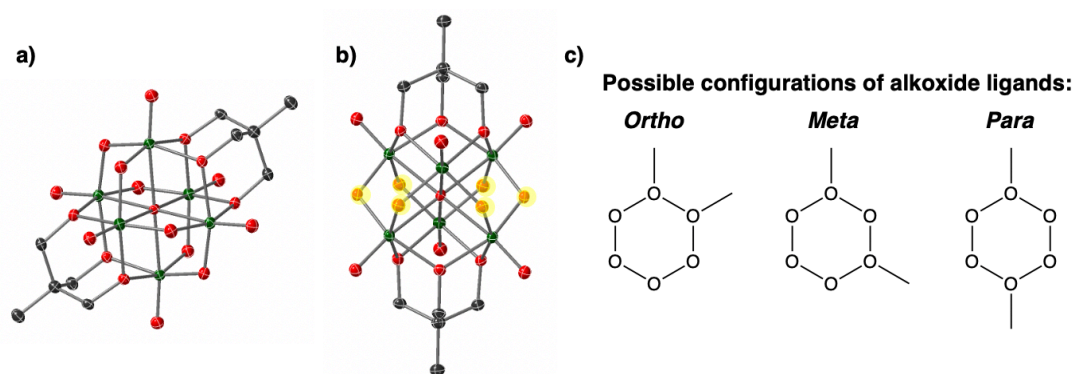
Figure 4. a) Molecular structure of POV-alkoxide cluster shown in typical view, red ellipsoids: O, dark green ellipsoids: V, dark grey ellipsoids: C; b) rotation of POV-alkoxide cluster to highlight the belt of six bridging oxido ligands; note that \mu_2\text{-O}^{2-} moieties available for surface functionalisation are highlighted in yellow; c) possible relative positions of new alkoxy ligands in bis-functionalised POV-alkoxide clusters.
