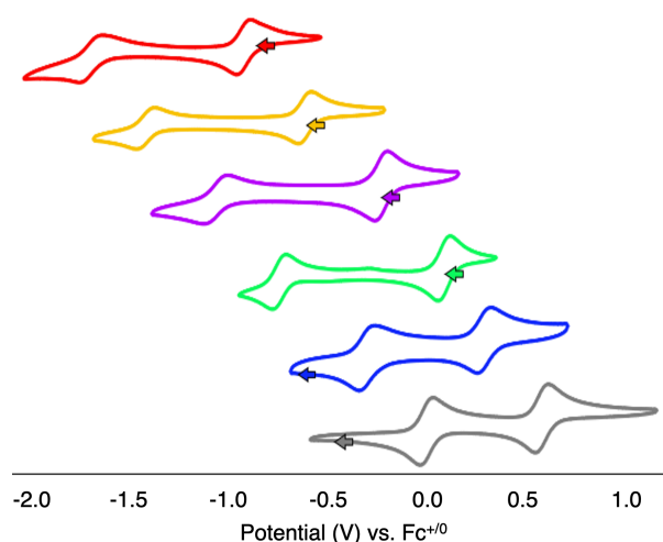
Figure 6. Cyclic voltammograms of complexes 1 (red, top), 2 (orange), 1-OMe (purple), 2-OMe (green), 1-(OMe) 2 (blue), and 2-(OMe) 2 (gray, bottom). All voltammograms were collected using 1 mM solutions of the complexes in acetonitrile with 0.1 M [\text{nBu}_4\text{N}][\text{PF}_6] as the supporting electrolyte at a scan rate of 200 mV/s.
