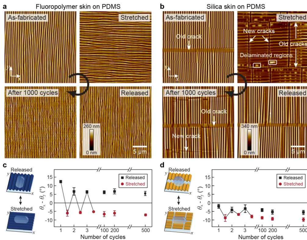
Figure 2. Crack-free nanowrinkles with switchable orientation enabled by plasma-mediated soft skin layers. Side-by-side comparison of wrinkle topography of (a) fluoropolymer and (b) silica skin wrinkles under stretch-release cycles. Anisotropic wetting on wrinkled (c) fluoropolymer and (d) silica skin layers. Adapted with permission from ref 33. Copyright 2017 John Wiley and Sons.
