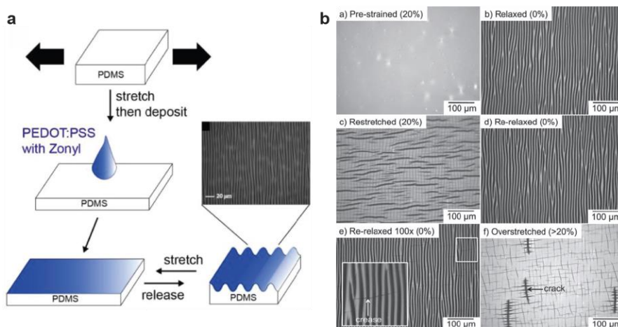
Figure 1. Mechano-responsive patterns from wrinkling solution-processed polymer skin layers. (a) Fabrication of polymer wrinkles based on spin-coating. (b) Structural evolution of wrinkled organic semiconductor film at different strains. Panel a adapted with permission from ref 37. Copyright 2019 John Wiley and Sons. Panel b adapted with permission from ref 30. Copyright 2011 John Wiley and Sons.
