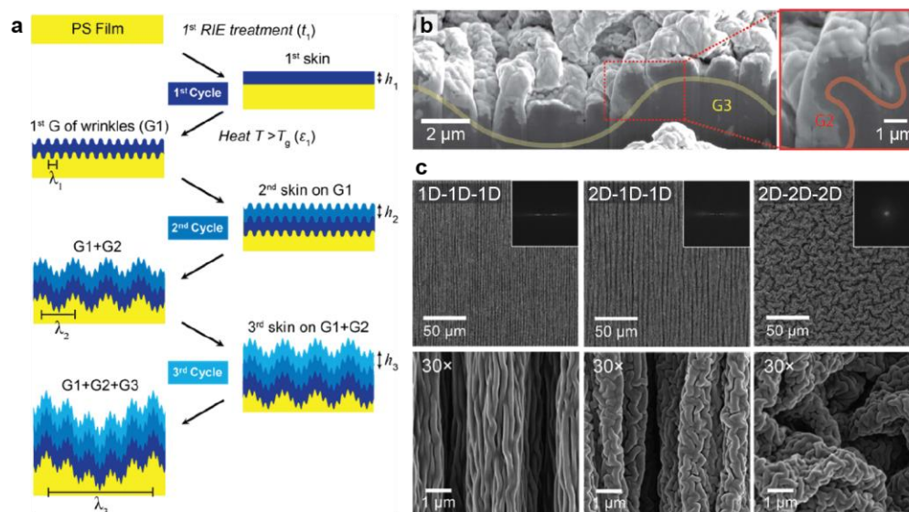
Figure 5. Multigenerational, hierarchical structures from sequential wrinkling of plasma-mediated soft skin layers. (a) Design principles of sequential process. (b) Conformal interface between skin layers and substrate. (c) Hierarchical wrinkles from three cycles of sequential skin growth and strain relief. Adapted with permission from ref 34. Copyright 2015 American Chemical Society.
