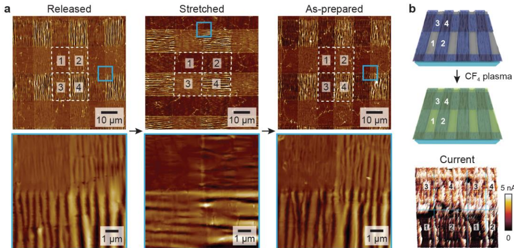
Figure 4. Multiscale graphene wrinkles with spatially defined structural features and properties. (a) Graphene patterned with four regions with different wavelengths. (b) Spatially defined electrical conductivities after plasma functionalization. Panel a adapted with permission from ref 55. Copyright 2020 American Chemical Society. Panel b adapted with permission from ref 72. Copyright 2019 American Chemical Society.
