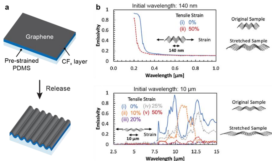
Figure 3. Conformal graphene wrinkles for tunable emissivity. (a) Scheme describing conformal wrinkling of graphene on fluoropolymer-coated PDMS. (b) Emissivity of nanotextured graphene with different feature sizes. Panel a adapted with permission from ref 55. Copyright 2020 American Chemical Society. Panels b adapted with permission from ref 70. Copyright 2019 American Chemical Society.
