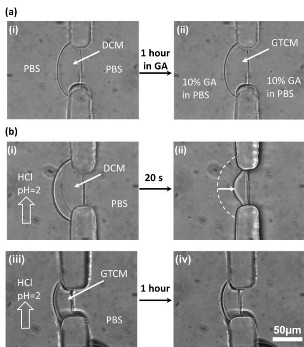
Figure 3. GA crosslinking and acidic resistance of DCM & GTCM. (a) No obvious morphology changes after soaking DCM in 10% GA in PBS for one hour to convert it into GTCM. (b) -(i) & (ii) DCM was dissolved by HCl (pH=2) solution in seconds, while (iii) & (iv) No change in GTCM was observed in the same condition for one hour.
