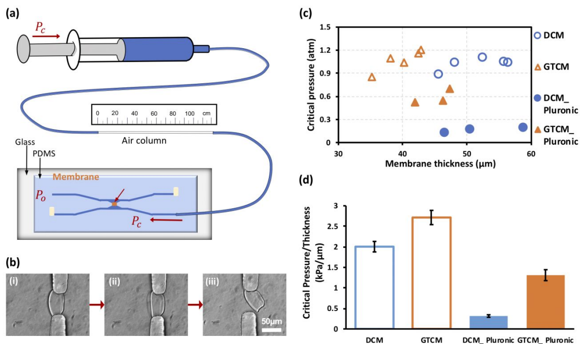
Figure 4. Mechanical robustness of DCM and GTCM. (a) Schematic of measurement setup based on Ideal Gas Law to measure the critical pressure to detach membranes between PDMS pillars. (b) Membrane (i) before, (ii) during and (iii) right at the burst moment during a robustness test. (c) Critical pressure of membranes when burst and those after Pluronic treatment. (d) Normalized critical pressure per \mu\text{m} thickness for different membranes.
