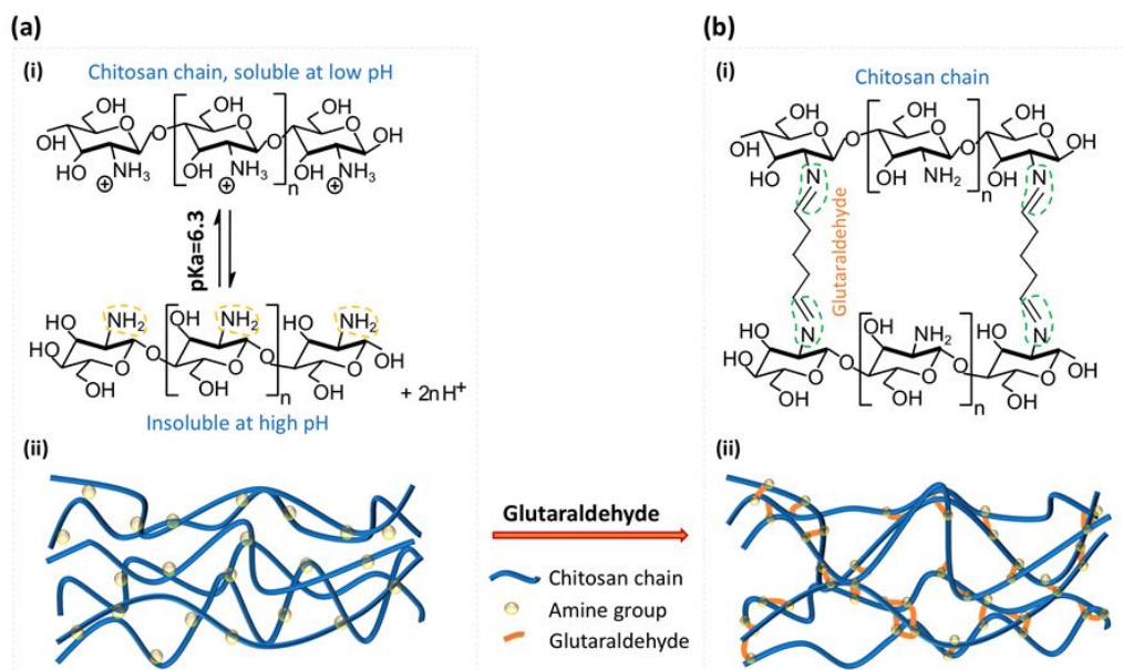
Figure 1. The molecular schematic of deprotonated chitosan membrane (DCM) cross-linked with glutaraldehyde. (a)-(i) Transition between protonated (soluble) and deprotonated (insoluble) chitosan around its \text{pK}_a value 6.3; (ii) Molecular structure of DCM with deprotonated amine groups. (b)-(i) The most commonly recognized molecular reaction between amine groups on DCM and glutaraldehyde (GA) molecules; and (ii) Molecular structure of glutaraldehyde treated chitosan membrane (GTCM) with GA linking between amine groups on nearby chitosan chains or within one chitosan chain.
