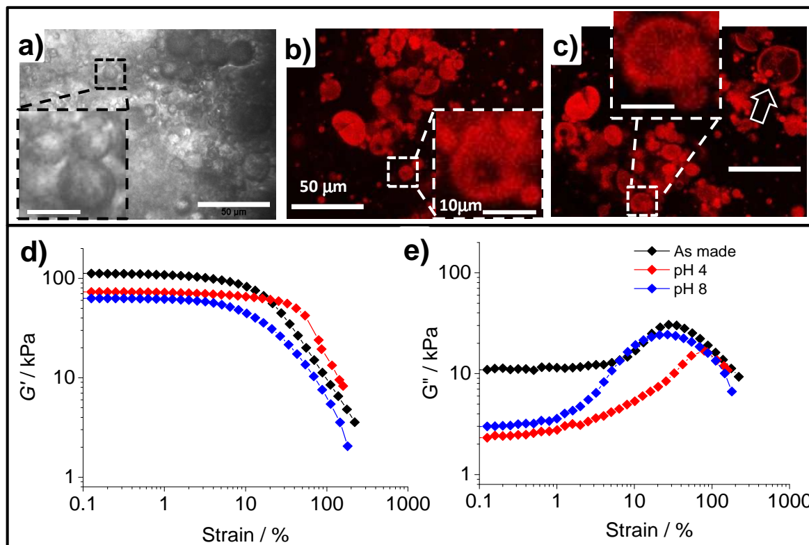
Fig. 8. Morphology and mechanical properties at different pH values. Optical microscopy (a) and CLSM images (b and c) for as-made (a) and PAAM/HP XL(10) gels at pH 4.0 (b) and 8.0 (c), respectively. The scale bars in (b) also apply to (a) and (c). The arrow in (c) highlights a large hollow particle. (d) and (e) show strain-sweep rheology data for PAAM/HP XL(20) gels before and after swelling equilibrium at pH 4.0 and 8.0.
