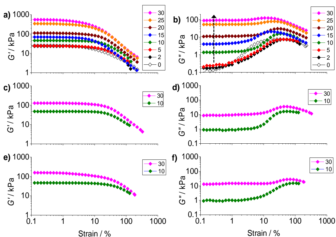
Fig. 5. Strain-sweep rheology study. Data for G' (left column) and G'' (right column) are shown as a function of strain for PAAm/HP XL(y) (a and b), PAAm/HP VF(y) (c and d) and PAAm/HP (y) (e and f). The values for y are shown in the legends. The arrow in (b) highlights the increase for G'' at low strain with increasing y .
