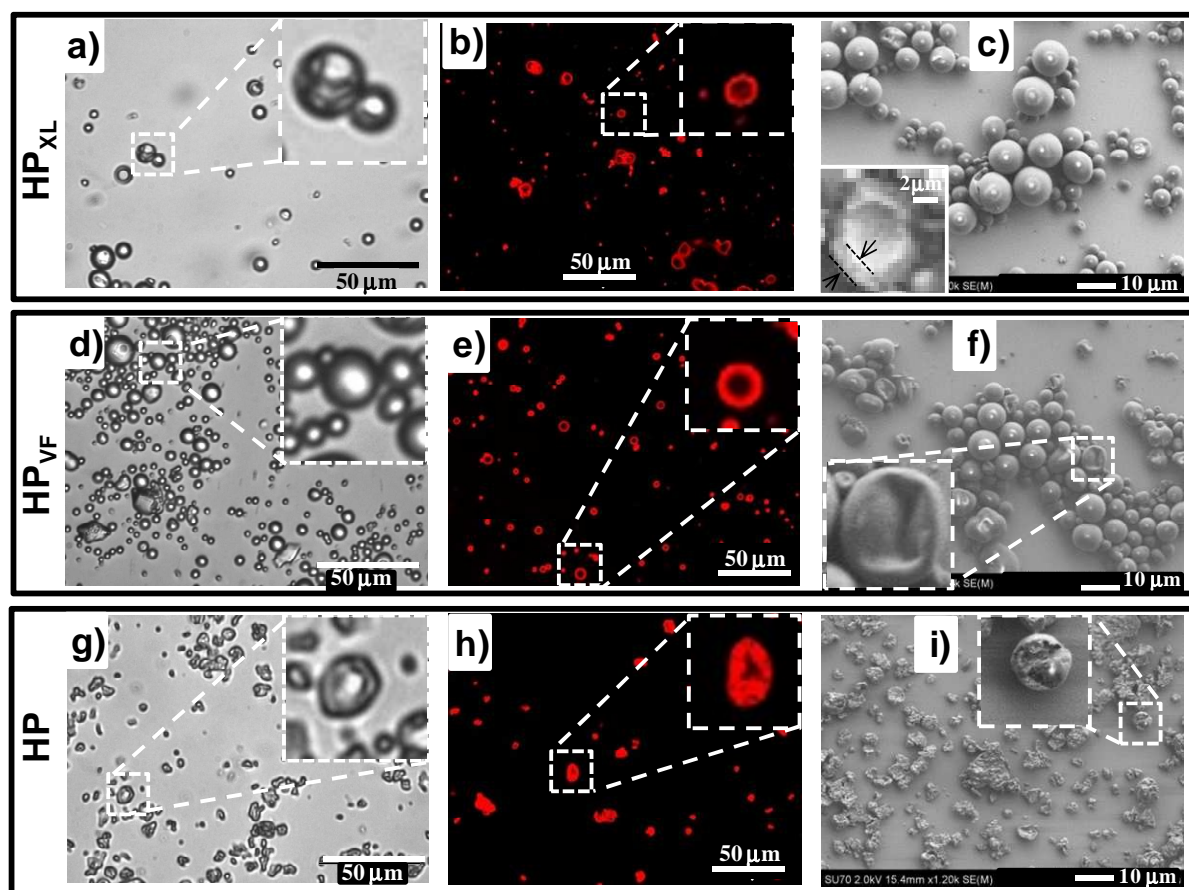
Fig. 1: Hollow particle morphologies. The identities of the hollow particles are shown in the left hand side of each row. Images from optical microscopy (left hand column) as well as CLSM (middle column) and SEM (right hand column) are shown. The pH of the dispersions was \sim 5.6 for all systems.
