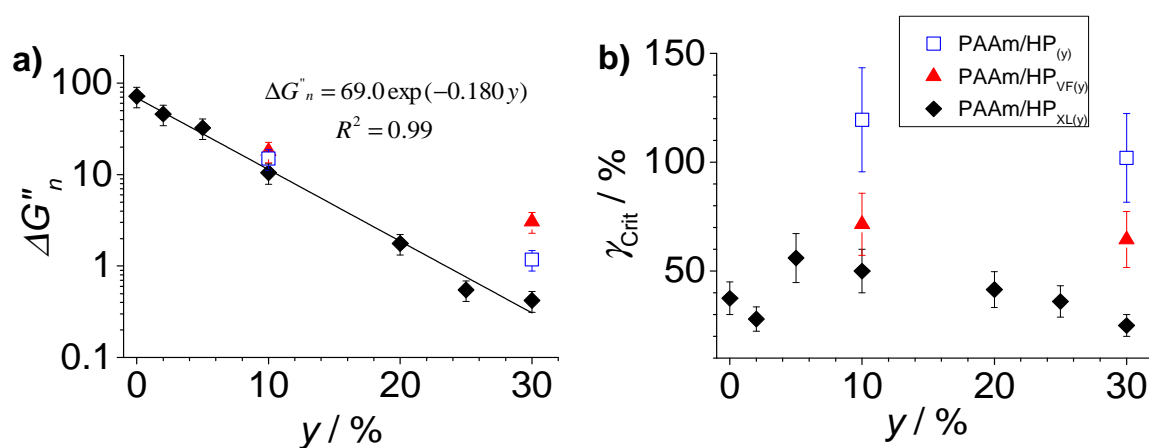
Fig. 6. Effects of particle concentration on gel dissipation and ductility. (a) Variation of \Delta G''_n ( = (G''_{peak} - G''_o)/G''_o ) where G''_{peak} and G''_o are maximum G'' and strain-independent G'' values, respectively) and (b) Variation of \gamma_{crit} with particle concentration ( y ) for the composite gels. The data have been taken from Fig. 5.
