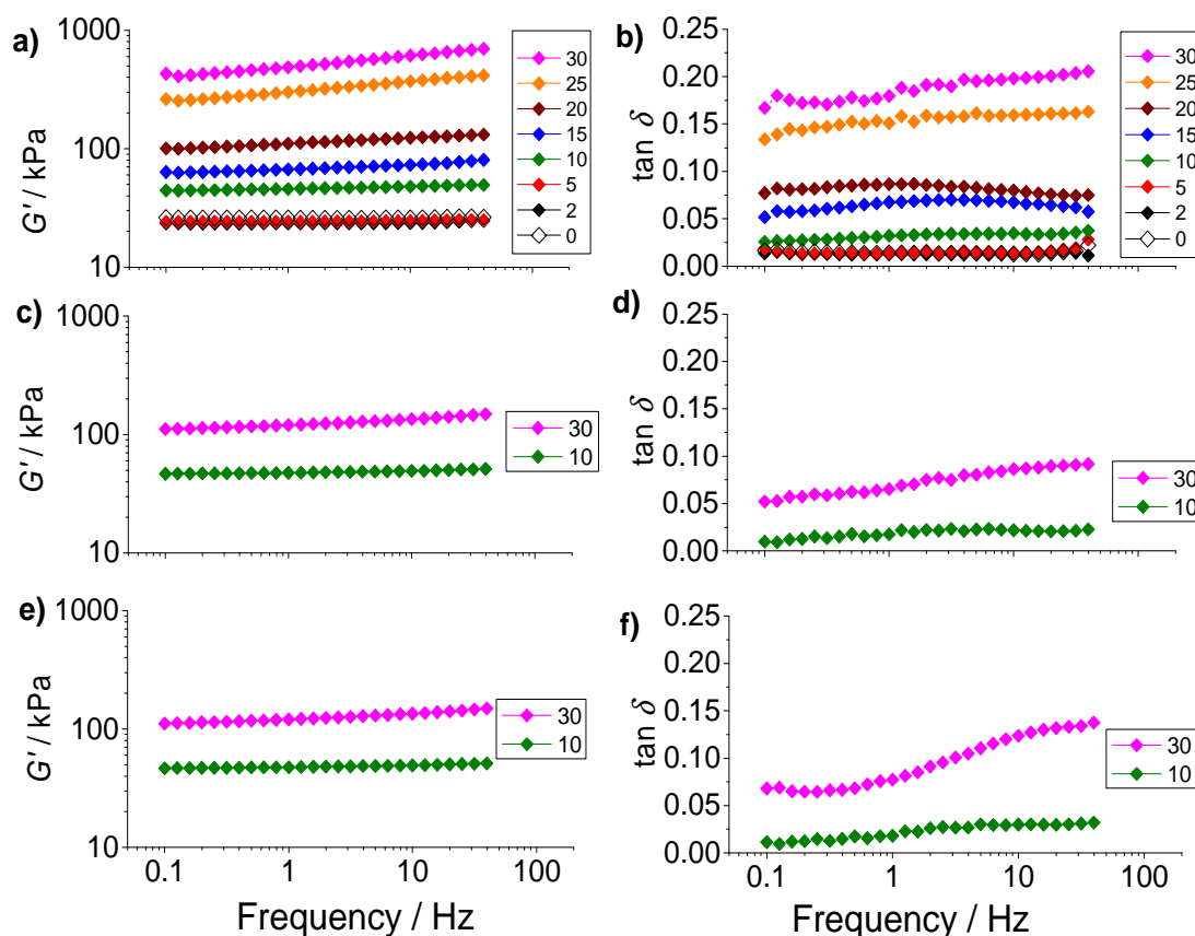
Fig. 3. Frequency-sweep rheology study. The variations of G' (storage modulus) and \tan\delta ( = G'' / G' , where G'' is the loss modulus) with frequency are shown in the left and right columns, respectively, for PAAm/HP XL(y) (a and b), PAAm/HP VF(y) (c and d) and PAAm/HP (y) (e and f). The legends show the values for y (%).
