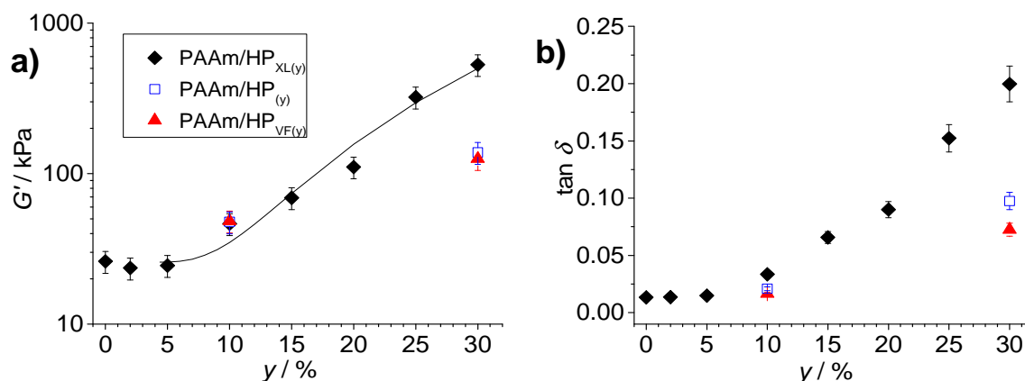
Fig. 4. Effects of hollow particle concentration on gel mechanical properties. The variations of (a) G' and (b) \tan \delta with particle concentration ( y ) are shown for the three composite gels. The data have been taken from Fig. 3. The legend applies to both graphs. The curve in (a) is the fit from equation 1. The value for A was 0.10.
