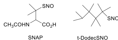
Figure 1- Structures of S-nitroso-N-acetylpenicillamine (SNAP) and S-nitroso-t-dodecanethiol (t-DodecSNO).
