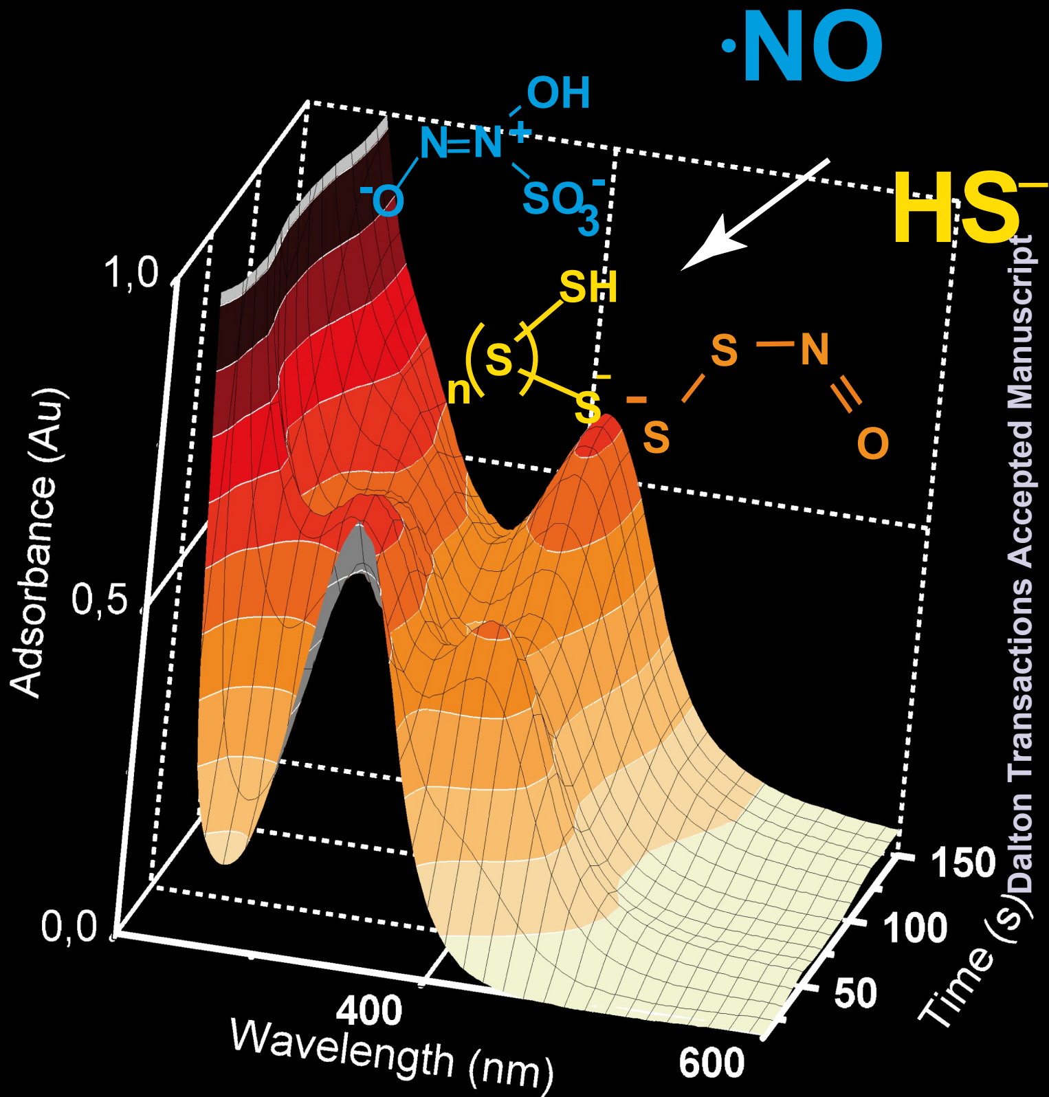
UV-visible spectral changes during the reaction of 1 mM SNAP with 4.5 mM Na 2 S in TRIS at pH 7.4
