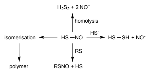
Figure 2. Reactivity of HSNO formed by the reaction of RSNO and HS - : isomerization, homolysis, nucleophilic attack and transnitrosation
