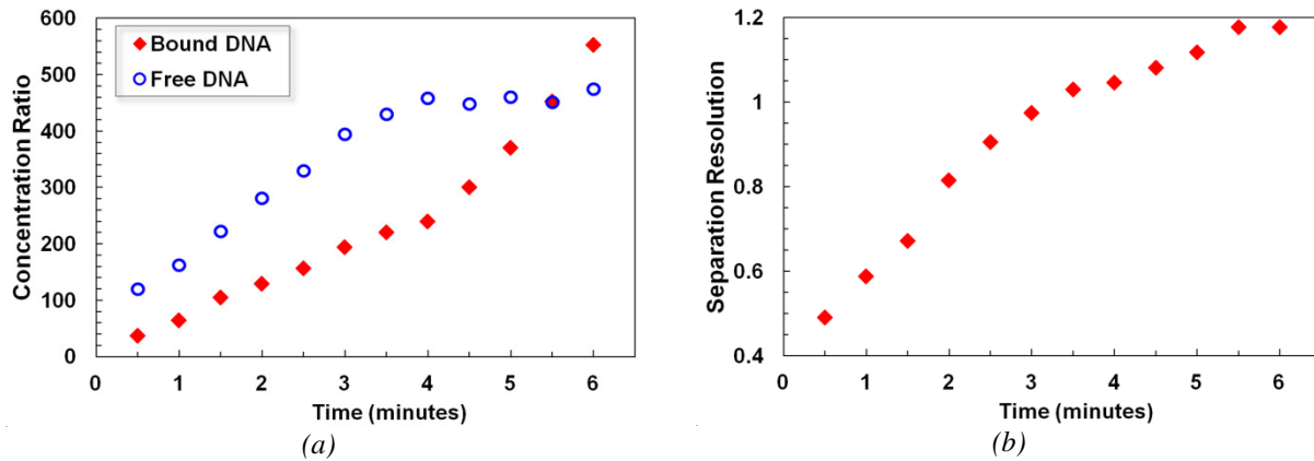
Figure 4. Quantitative performance analysis of the dual-channel microfluidic BPE: (a) Concentration ratio vs. time. The concentration speed for bound DNA is lower due to the larger size; and (b) Separation resolution vs. time.
