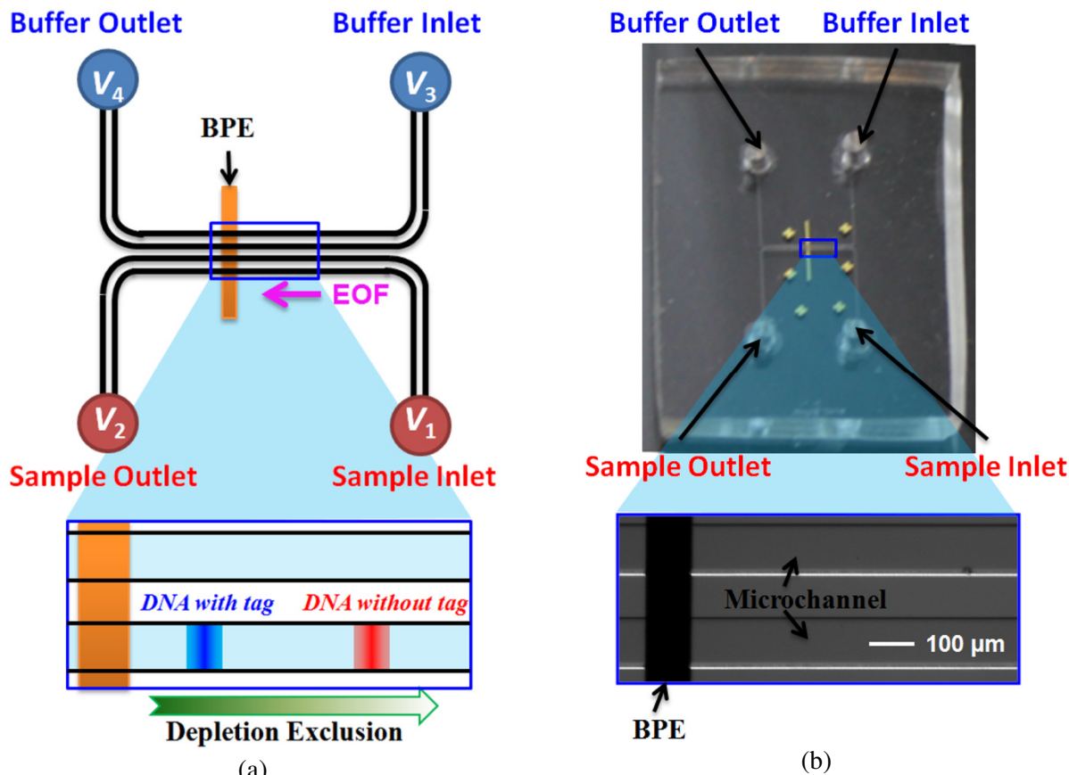
Figure 1. (a) Schematic of dual-channel microfluidic BPE device. The top channel is used to load the buffer and the bottom channel is used to load the DNA containing samples. A single bipolar electrode (BPE), located at the floor of the channels, intersects both channels; and (b) The assembled device with an enlarged view of the BPE-microchannel junction. The electrode is fabricated using standard lithography with chrome/gold on glass. The fluidic channels are made out of PDMS using soft lithography.
