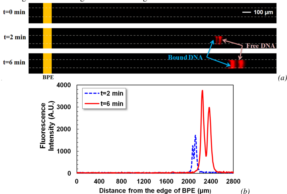
Figure 3. Concurrent concentration and separation of the free DNA and the bound DNA in the present dual-channel microfluidic BPE device: (a) Fluorescence images at different times points; and (b) Fluorescence intensity along the channel
