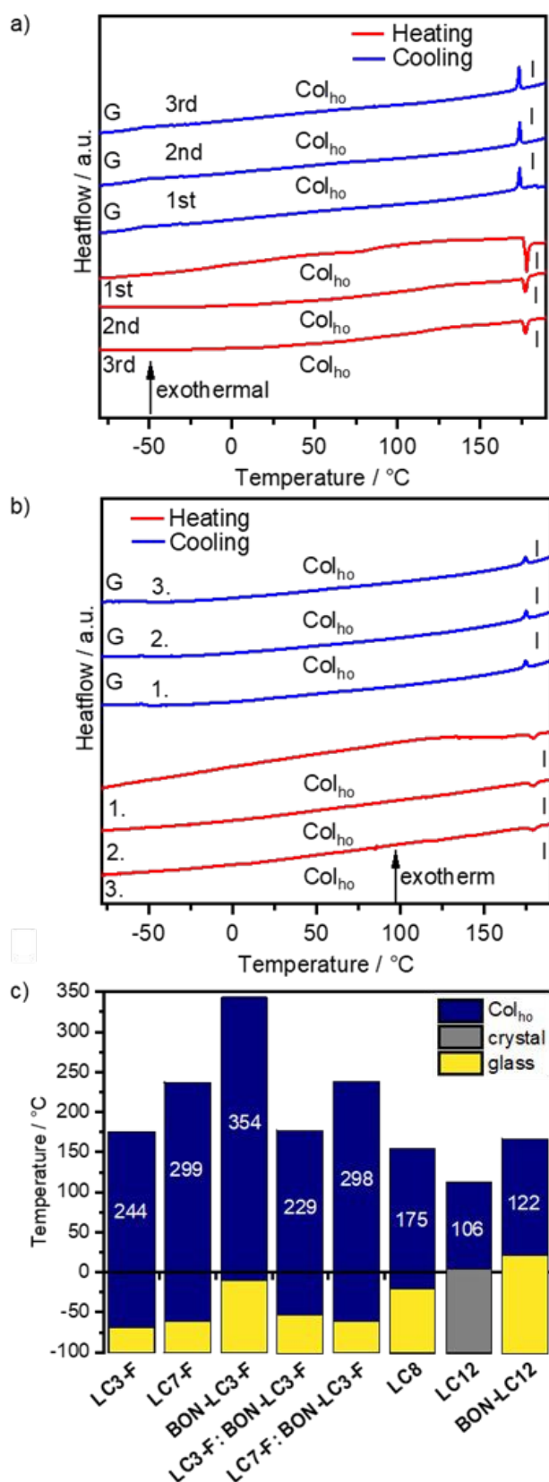
Figure 2. a) DSC thermogram (heating/cooling rate: 10 \text{ K} \cdot \text{min}^{-1} ) of compound LC3-F . G = glassy state, Col ho : columnar hexagonally ordered mesophase, I = isotropic melt; b) DSC thermogram (heating/cooling rate: 10 \text{ K} \cdot \text{min}^{-1} ) of LC3-F doped with 1 wt% of BON-LC3-F ; c) Phase ranges of the semi-perfluorinated derivatives LC3-F , LC7-F , BON-LC3-F as well as mixtures LC3-
