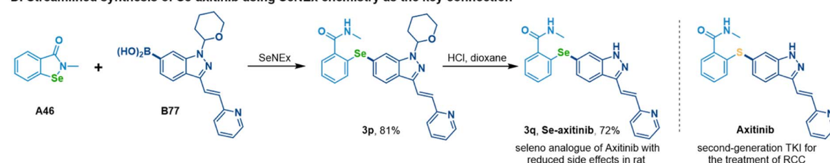
Fig. 3 Diversified synthetic application of this SeNEx chemistry. (A) The orthogonal reactivity of SeNEx to ArI, COOH, NH 2 , indole and N 3 -based elaboration. (B) The orthogonal reactivity of SeNEx with SuFEx and CuAAC catalysis. (C) A purification-free click chemistry sequence of SeNEx-SuFEx-SuFEx. (D) Streamlined synthesis of seleno-axitinib by using SeNEx chemistry as the key connection.
