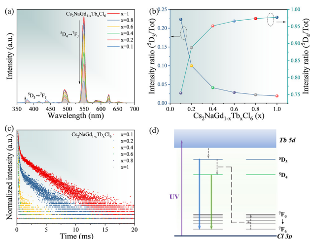
Fig. 2 (a) PL spectra of Cs_2NaGd_{1-x}Tb_xCl_6 under an excitation wavelength of 275 nm. (b) The emission ratio from {}^5D_3 and {}^5D_4 levels over total emission. (c) Photoluminescence decay curves for the {}^5D_3 level (437 nm). (d) Energy-level diagram for Tb^{3+} ions in Cs_2NaGd_{1-x}Tb_xCl_6 showing a possible route of luminescence quenching and cross-relaxation.
