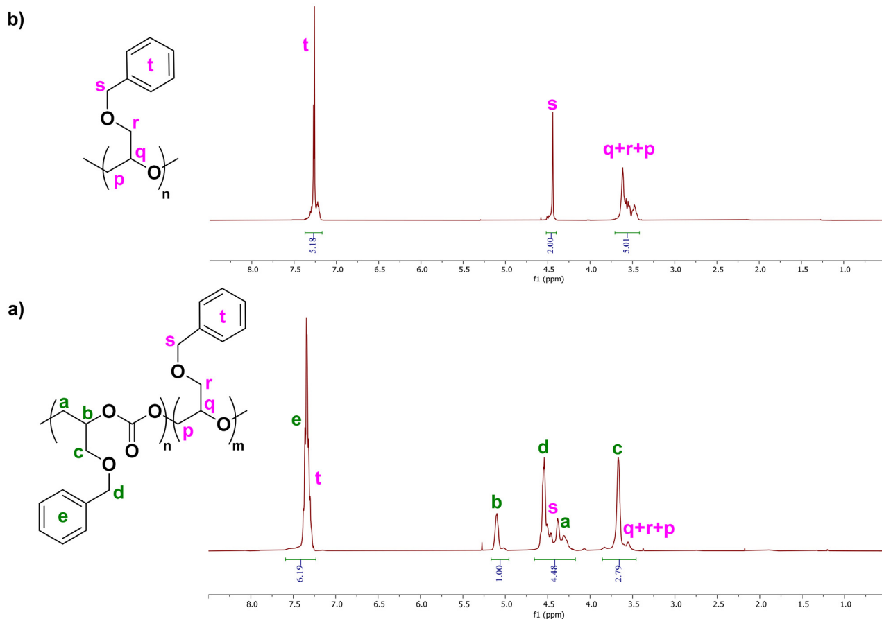
Fig. 1 Representative ^1\text{H} NMR (400 MHz, \text{CDCl}_3 , 23 ^\circ\text{C} ) spectra of PBnGEC with minor ether linkages (a)-bottom, and pristine PBnGEE (b)-top prepared with the \text{BEt}_3 /PPNCl catalyst system.
