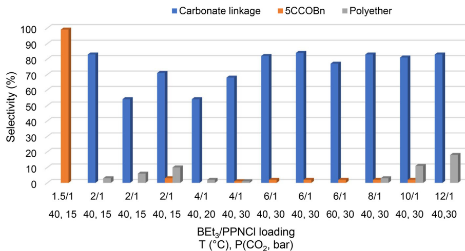
Fig. 2 Effects of the \text{BEt}_3 /PPNCl ratio, reaction temperature and \text{CO}_2 pressure on the selectivity of the \text{CO}_2 /BnGE ROCOP (Table 2).
