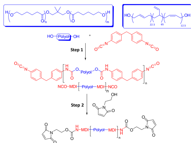
Scheme 2 Synthesis of bismaleimide PU prepolymers. Step (1) bulk, 110\text{ }^\circ\text{C} for 1 hour. Step (2) bulk, 120\text{ }^\circ\text{C} for 1.5–2 hours.
