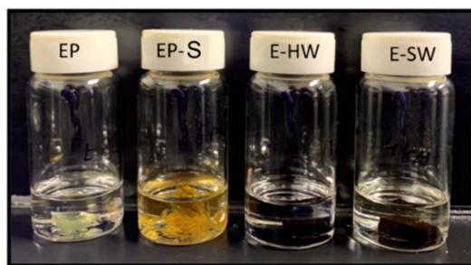
Fig. 7 Immersed epoxy thermosets in tetrahydrofuran. E-SW: epoxidized softwood, E-HW: epoxidized hardwood, EP-S: epon/ethyl lactate, EP: epon.
