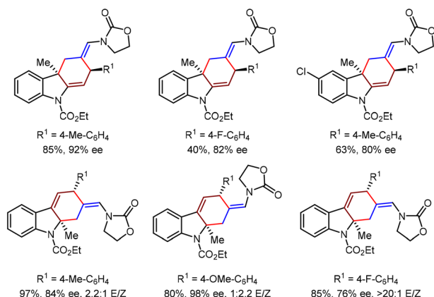
Scheme 37 Au(I)/DTBM-Segphos-catalyzed asymmetric dearomative [4+2] cycloadditions of 3/2-substituted 2/3-vinylindoles and N -allenamides.
