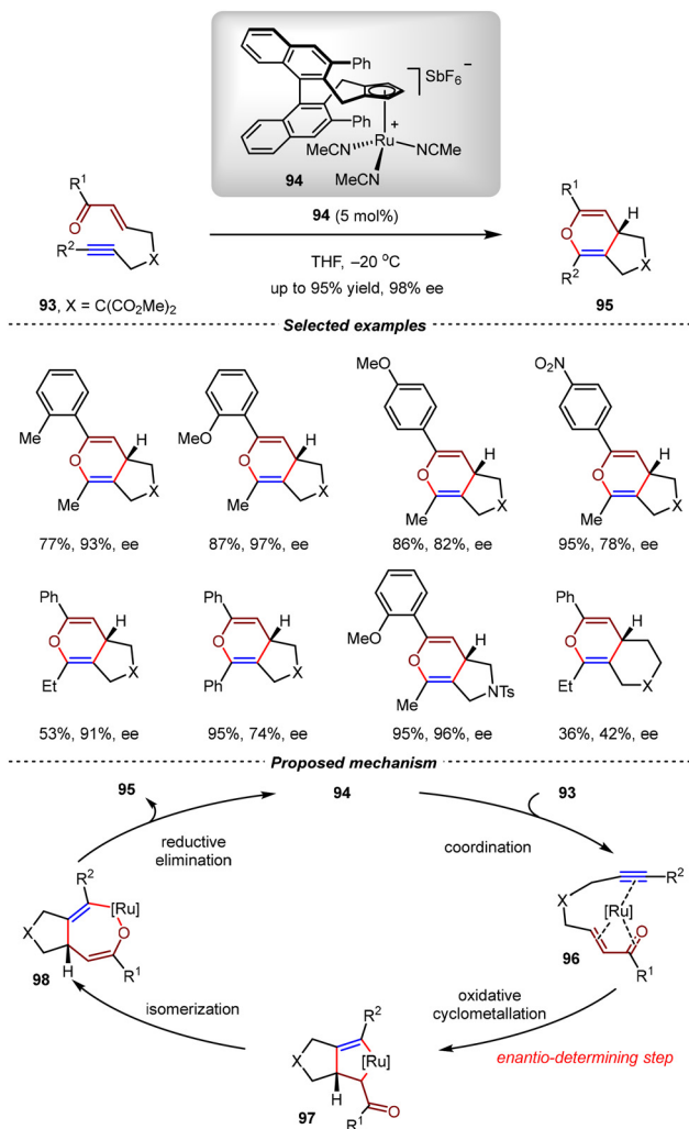
Scheme 24 Ruthenium (II)-catalyzed asymmetric intramolecular [4+2] cycloadditions of yne-enones.
