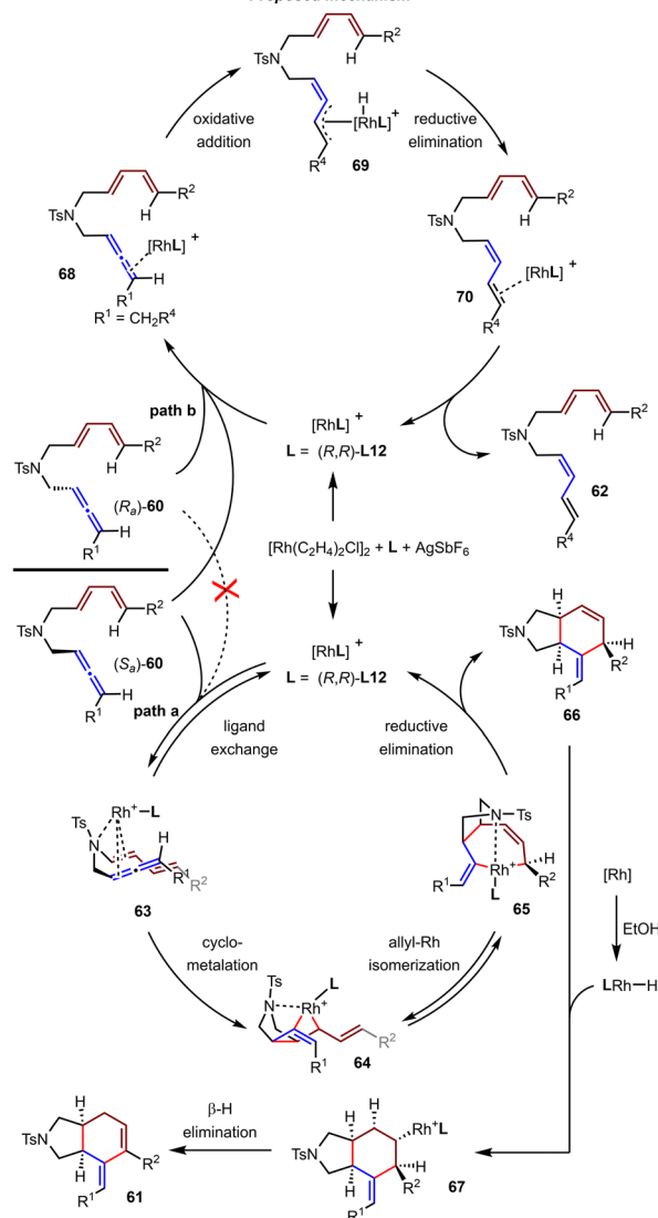
Scheme 18 Rh(I)/Ph-BPE-catalyzed kinetic resolution of racemic 1,3-disubstituted allene-1,3-dienes.
