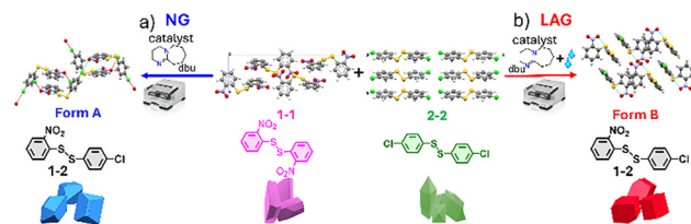
Fig. 6 Model reaction used to probe ball milling trends. Base-catalysed (DBU) disulfide exchange between equimolar 1-1 and 2-2 yields the heterodimer 1-2 . (a) Neat grinding (NG) produces polymorph Form A. (b) Liquid-assisted grinding (LAG) produces polymorph Form B. 41
