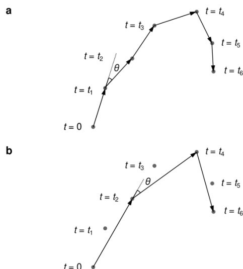
Figure 2. Definition of directionality. a , The trajectory of a particle assessed using microscopy. The (approximate) location of the particle (dots) is sampled at discrete times t = t_1, t_2, \text{etc.} Between each pair of such sampled locations we can form a displacement vector (arrows) and define the change in direction (angle \theta ) between displacements. b , It is also possible to follow the change in direction (angle \theta ) over longer time-intervals, in this case between every other frame.
