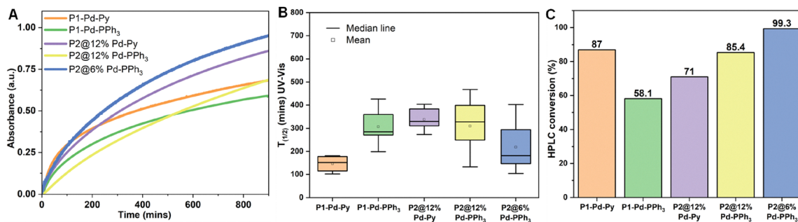
Fig. 2 (A) Kinetic profiles of encapsulated P1 and covalently attached P2 NPs in a pro-DNP ( 4 ) (100 μM) to DNP ( 5 ) conversion monitored by UV-Vis over time at λ = 400 nm in water at 37 °C using 30 μM of Pd; (B) T 1/2 comparison of the P1 and P2 NPs in the formation of DNP ( 5 ); T 1/2 (time taken for 50% formation of DNP ( 5 ) by UV-Vis, mean of multiple runs); (C) HPLC conversion of DNP ( 5 ) after 24 h.
