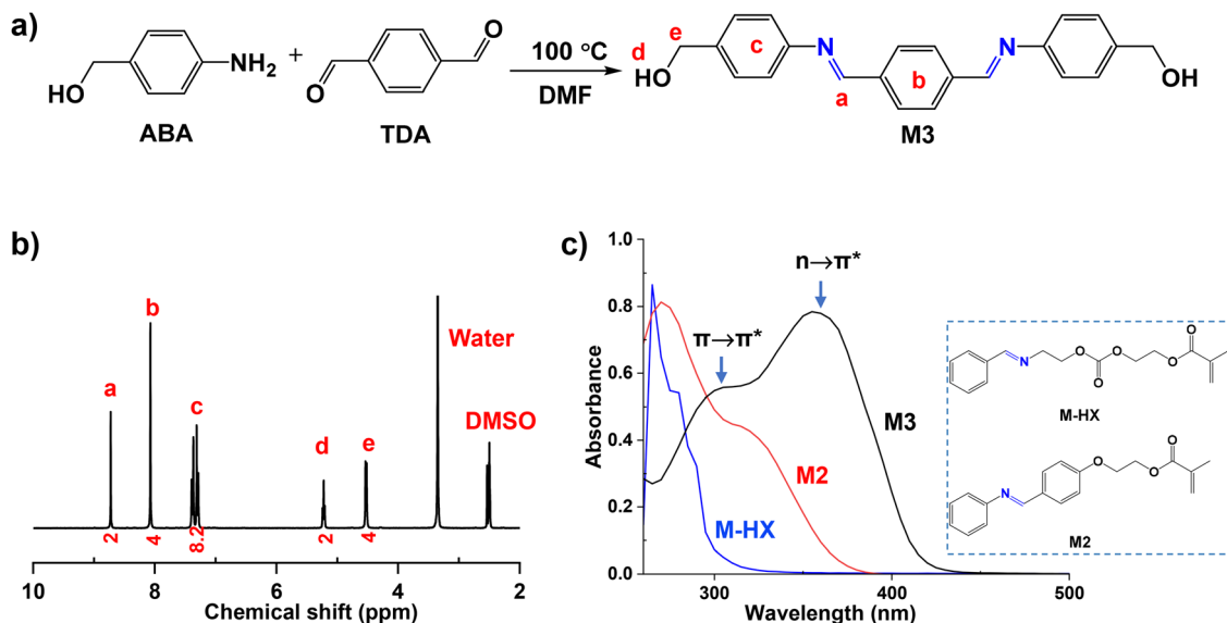
Fig. 1 Synthesis of M3 (a diol crosslinker bearing an extended conjugate benzoic imine) through the condensation reaction of ABA with TDA in DMF (a), its ^1\text{H} NMR spectrum in DMSO- d_6 (b), and its UV/vis spectrum in DMSO, compared with those of M2 (a methacrylate bearing a conjugate benzoic imine bond) and M-HX (a methacrylate bearing a benzoic imine bond) in DMF (c).
