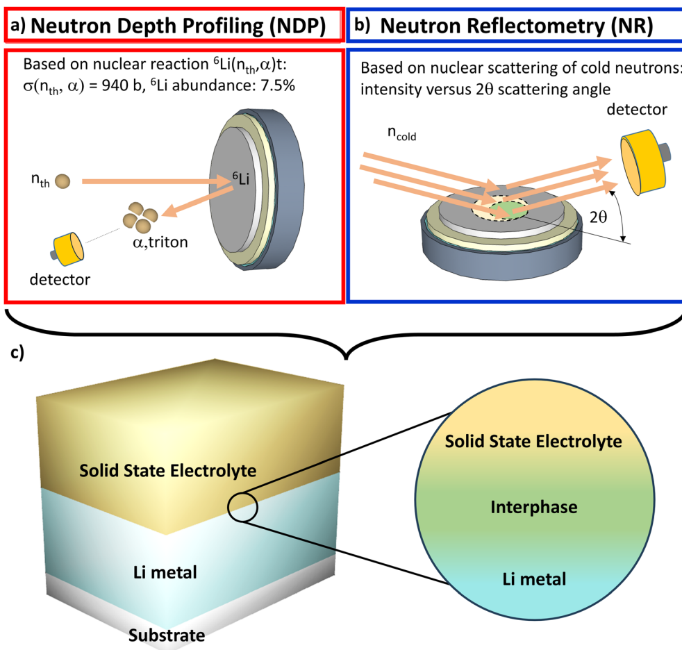
Fig. 1 a) Schematic illustration of neutron depth profiling (NDP) where thermal neutrons ( n_{th} ) penetrate a sample and react with ^6\text{Li} producing both \alpha and Triton radiation which are then measured. (b) Schematic illustration of neutron reflectometry (NR) where cold neutrons ( n_{cold} ) reflect and refract through a thin film multilayer forming a reflected neutron spectra with both constructive and destructive interference resulting in a Kiessig fringe pattern on the detector. (c) Schematic illustration of a typical sample consisting of a solid electrolyte connected (SSE) paired with a Li metal electrode. The blowout highlights the formation of an interphase between the solid electrolyte and the Li metal which can be studied with both NDP and NR.
