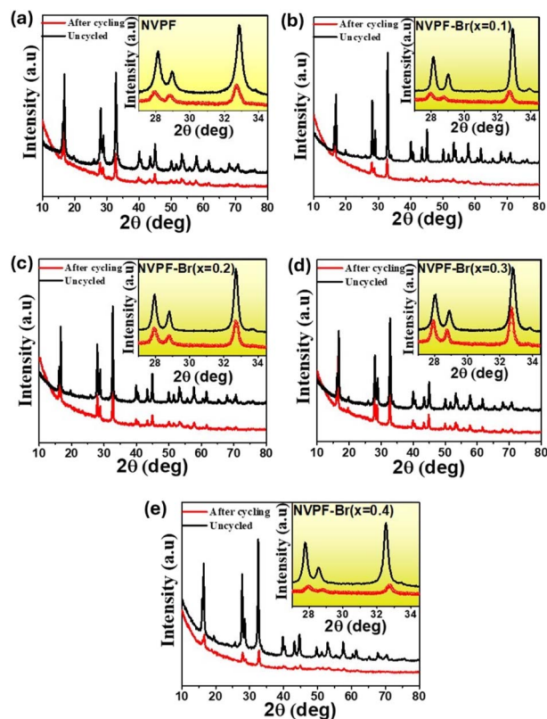
Fig. 7 Post-cycling XRD spectra of cathodes. (a) NVPF, (b) NVPF-Br ( x = 0.1 ), (c) NVPF-Br ( x = 0.2 ), (d) NVPF-Br ( x = 0.3 ), and (e) NVPF-Br ( x = 0.4 ). Insets show the magnified 2\theta region.
