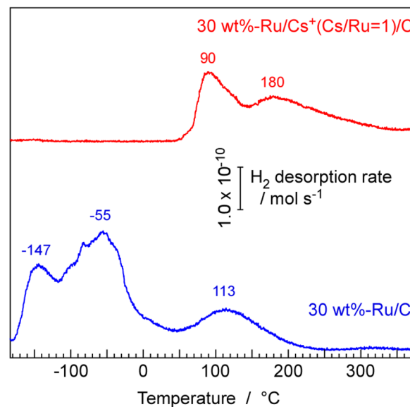
Fig. 10 TPD spectra of H 2 from 30 wt%-Ru/C and 30 wt%-Ru/Cs + /C (Cs + /Ru = 1 : 1)/C. The ramping rate of temperature was 10 °C min -1 . The samples were treated by reduction treatment at 400 °C, followed by evacuation at 400 °C, prior to TPD measurements. The adsorption of H 2 was performed at -183 °C and 5.0 kPa.
