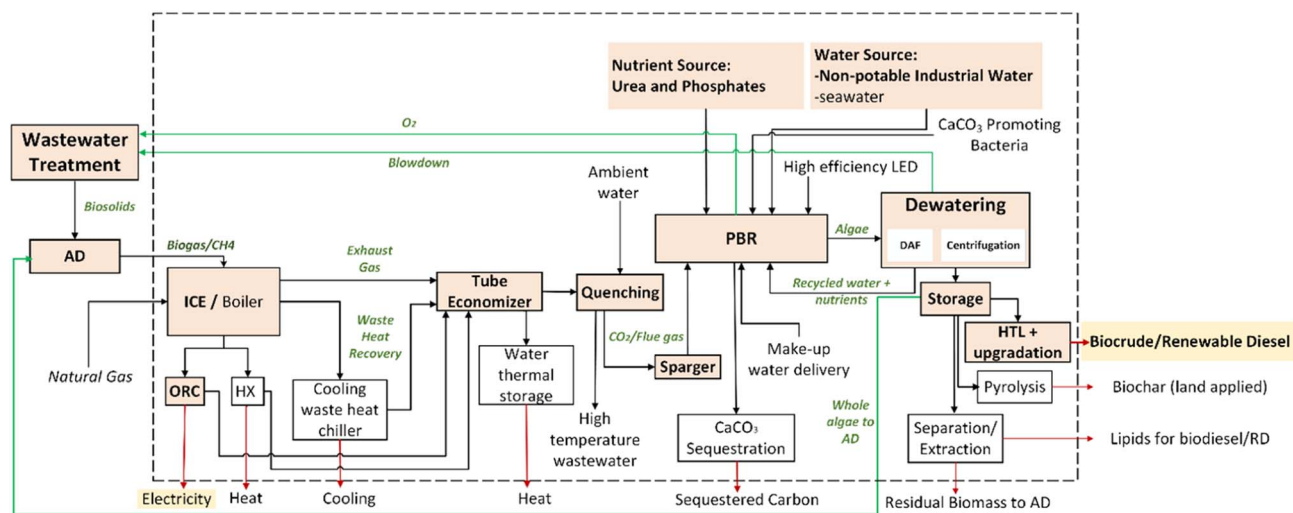
Fig. 1 System boundary for the LCA and TEA baseline and sensitivity configurations evaluated in the study. The baseline configuration is shown via colored boxes with bold text, while the sensitivity cases are shown in monochromatic boxes. Green arrows pertain to the reuse/recycle of resources. AD – Anaerobic Digestion, ICE – Internal Combustion Engine, ORC – Organic Rankine Cycle, PBR – photobioreactor, HTL – hydrothermal liquefaction, HX – heat exchanger, LED – Light Emitting Diode, DAF – Dissolved Air Flotation, \text{CaCO}_3 – calcium carbonate, \text{O}_2 – oxygen gas, and RD – Renewable Diesel.
