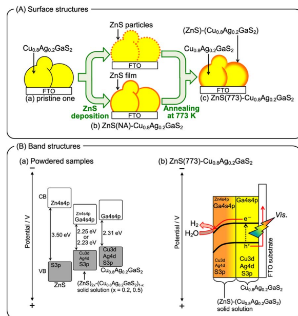
Fig. 4 (A) Proposed surface structures of the particulate-Cu 0.8 Ag 0.2 GaS 2 -based photocathode, and (B) proposed band structures of (ZnS) 2x –(Cu 0.8 Ag 0.2 GaS 2 ) 1-x powders and the ZnS(773)–Cu 0.8 Ag 0.2 GaS 2 photocathode. The band gaps were estimated from the adsorption edges shown in Fig. S4.†
