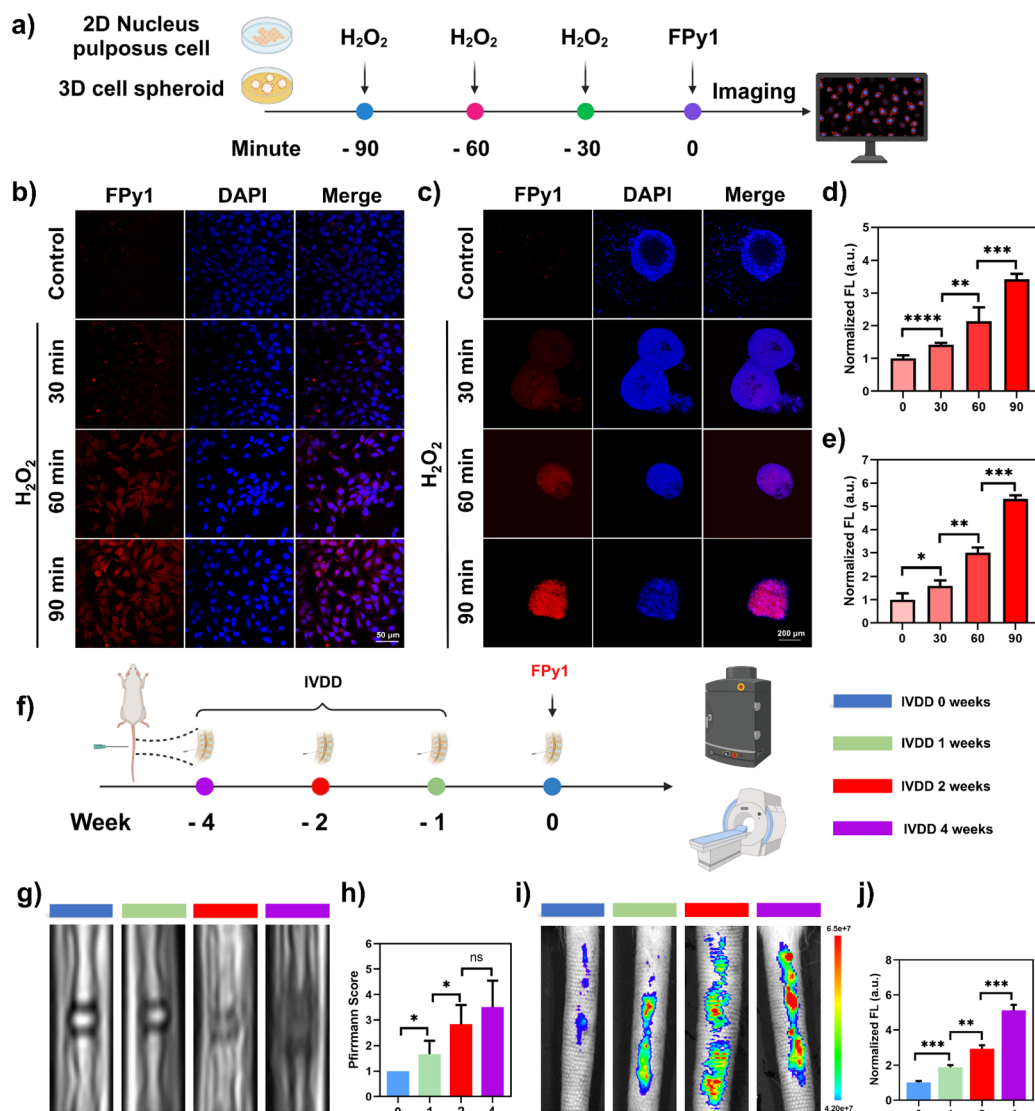
Fig. 4 Multi-scale bioimaging of Cas-1 in primary nucleus pulposus cells, cell spheroids and in vivo stained with FPy1 . (a) The illustration of fluorescence imaging in NP cells and spheroids stimulated by H_2O_2 (2 mM). (b) Confocal fluorescence images of NP cells stained with FPy1 (5 \mu M). First row, control group; second row, NP cells were stimulated with H_2O_2 for 30 min; third row, NP cells were stimulated with H_2O_2 for 60 min; fourth row, NP cells were stimulated with H_2O_2 for 90 min. FPy1 ( \lambda_{ex} = 514 nm, collected 530–610 nm); DAPI ( \lambda_{ex} = 405 nm, collected 420–470 nm). (c) Confocal fluorescence images of cell spheroids stained with FPy1 (5 \mu M). First row, control group; second row, spheroids were stimulated with H_2O_2 for 30 min; third row, spheroids were stimulated with H_2O_2 for 60 min; fourth row, spheroids were stimulated with H_2O_2 for 90 min. FPy1 ( \lambda_{ex} = 514 nm, collected 530–610 nm); DAPI ( \lambda_{ex} = 405 nm, collected 420–470 nm). (d) Quantitative analysis of fluorescence intensity in (b). (e) Quantitative analysis of fluorescence intensity in (c). (f) Scheme of fluorescence imaging or MRI in puncture-induced IVDD rat model. (g) Representative MRI images of intervertebral discs in rats at 0, 1, 2 and 4 weeks after puncture. (h) Pfirrmann grade from T_2 -weighted MRI in each group. (i) Fluorescence images of rat intervertebral discs at 0, 1, 2 and 4 weeks after puncture. (j) Quantitative analysis of fluorescence intensity in (i). Statistical analyses were performed with one-way ANOVA with multiple comparisons, the significance levels were donated as ns (not significant), * P < 0.05, ** P < 0.01, *** P < 0.001, and **** P < 0.0001.
