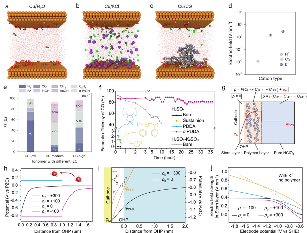
Fig. 11 Ionomers modulate the interfacial electric field in the electrocatalytic \text{CO}_2\text{RR} . MD-simulated atomic configurations of (a) \text{Cu}/\text{H}_2\text{O} , (b) \text{Cu}/\text{KCl} , and (c) \text{Cu}/\text{CG} systems at the end of NVE simulations ( \Delta U = 2.5 V). (d) Comparison of electric fields generated by \text{H}^+ , \text{K}^+ , and CG in the OHP. (e) Catalytic selectivity of Cu modified with CG-low, CG-medium, and CG-high in 0.2 M \text{H}_2\text{SO}_4 at 100 \text{mA cm}^{-2} . Reproduced with permission from ref. 36. Copyright 2023, Springer Nature. (f) FE for CO production on different ionomer-modified Ag catalysts at 200 \text{mA cm}^{-2} (electrolyte: 0.1 M \text{H}_2\text{SO}_4 ; bare Ag nanoparticle system used 0.4 M \text{K}_2\text{SO}_4 as an additive). (g) Simulation model: \rho denotes the total charge density; \rho_p represents the charge density carried by the ionomer layer. (h) Potential profiles on Ag electrodes covered by ionomer layers with different \rho_p values (unit: \text{C cm}^{-3} ) in 10 mM HOTf at -1.8 V vs. SHE. (i) Potential profiles on Ag electrodes coated with \rho_p = 300 \text{ C cm}^{-3} and \rho_p = 0 ionomer layers. (j) E_{\text{Stern}} versus electrode potential. Solid curves: Ag electrodes with different \rho_p ionomer layers (unit: \text{C cm}^{-3} ) in 10 mM HOTf. Gray dashed curve: the bare Ag electrode in 10 mM HOTf + 40 mM KOTf. Reproduced with permission from ref. 90. Copyright 2023, Springer Nature.
