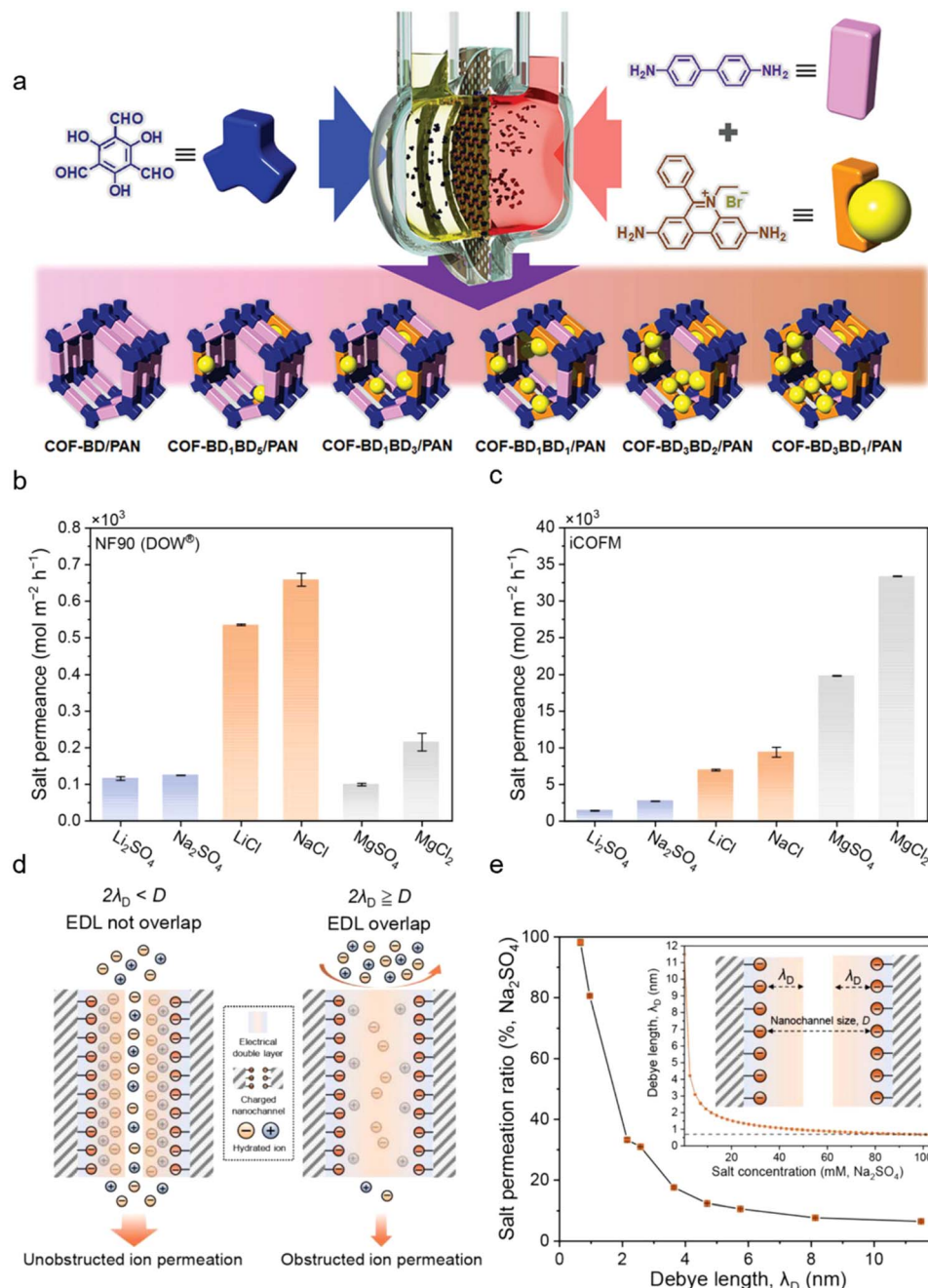
Fig. 6 (a) Schematic of charge density modulation through precise monomer ratio control. 57 Copyright 2021, Wiley-VCH. Ion transport behavior governed by the electric double-layer. Salt permeation rates of (b) commercial nanofiltration membranes versus (c) ionic COF membranes. (d) Electric double layer-governed ion diffusion behavior. (e) Salt permeability at varying Debye lengths. Insets: illustration of the Debye length–salt concentration correlation. 77 Copyright 2022, American Chemical Society.
