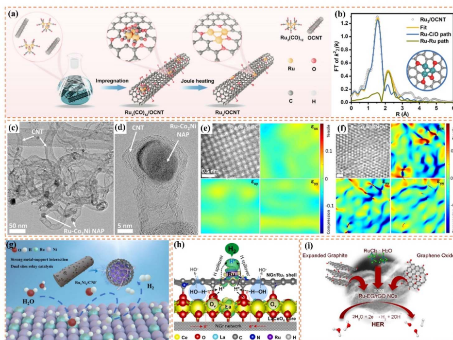
Fig. 8 (a) Schematic diagram of the synthesis of Ru 3 /OCNT catalyst. (b) Ru 3 /OCNT and d) Ru 1 /OCNT at R space. Inset: the schematic model of Ru 3 /OCNT and Ru 1 /OCNT. C: grey, O: red, and Ru: green. Reproduced with permission from ref. 114. Copyright 2025, Wiley-VCH. (c and d) HRTEM images of the Ru–Co 2 Ni@NCNT. Atomic resolution image along with the \epsilon_{xx} , \epsilon_{xy} , \epsilon_{yy} strain components determined via GPA of the (e) Ru–Co 2 Ni@C and (f) Ru–Co 2 Ni@NCNT. Reproduced with permission from ref. 125. Copyright 2025, Wiley-VCH. (g) Mechanism for enhancing the performance of Ru 1 Ni 6 /CNF. Reproduced with permission from ref. 126. Copyright 2025, Elsevier. (h) Possible hydrogen spillover mechanism for the alkaline HER over an advanced binary-site LaCeO x @NGr/Ru 1 catalyst. Reproduced with permission from ref. 128. Copyright 2024, Elsevier. (i) Mechanisms for Enhancing the Performance of Ru/EG-rGO NCs. Reproduced with permission from ref. 129. Copyright 2024, American Chemical Society.
