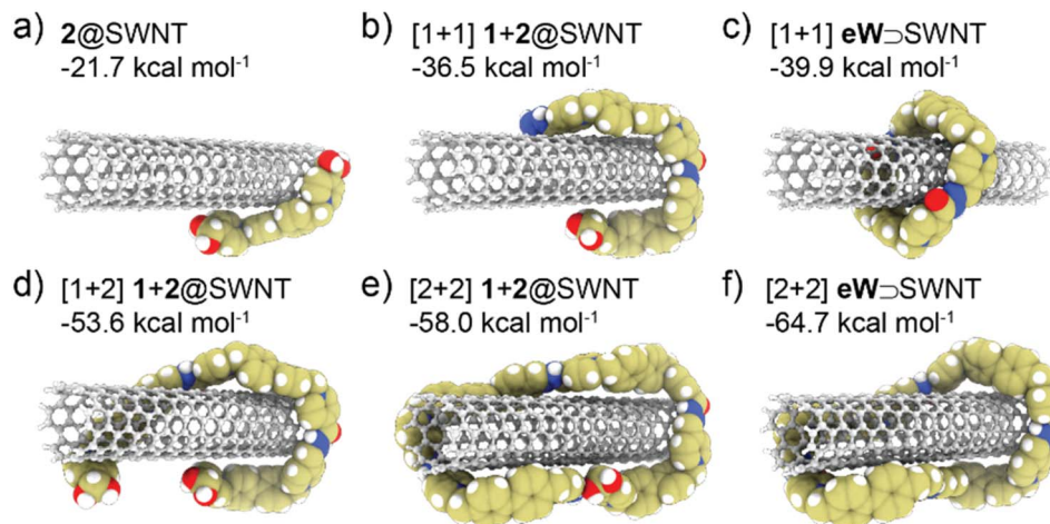
Fig. 6 Local minima and \Delta G_a values in \text{kcal mol}^{-1} computed at the \omega B97X-3c/SMD( \text{H}_2\text{O} )/GFN2/ALPB( \text{H}_2\text{O} ) level of theory, 16,17,22,23 for the potential aggregates formed by the association between a truncated hydrogen-capped section of a (6,5)-SWNT (ball-and-stick), and cyclic (c and f)/oligomeric (a, b, d and e) species arisen from the self-assembly of building blocks 1 and 2 (van der Waals spheres).
