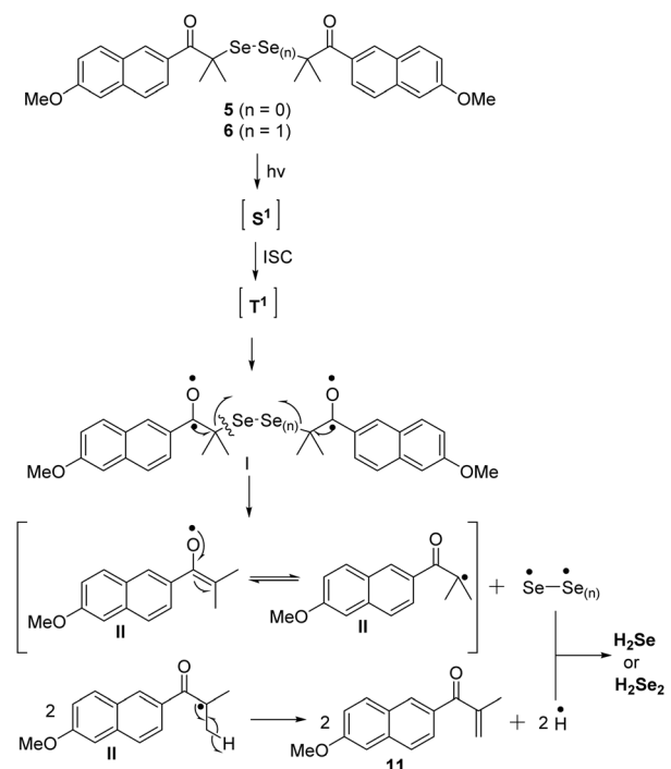
Scheme 11 Proposed mechanism of \text{H}_2\text{Se}_2/\text{H}_2\text{Se} formation from 5 and 6 .
