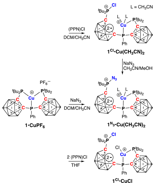
Scheme 5 Ligand-centered reactivity of [\text{tBuP-closo}\{-\text{C}_2\text{B}_{10}\}-\text{PhP}\}\text{-closo}\{-\text{C}_2\text{B}_{10}\}-\text{tBuP}]\text{CuPF}_6 ( 1 \cdot \text{CuPF}_6 ) with chloride and azide anions. Unlabeled cluster vertices represent BH units.
