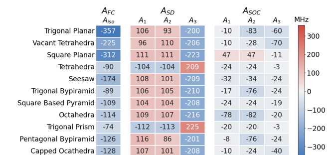
Fig. 9 Heatmap of computed V^{IV} HFC components for [V(NH_3)_x]^{4+} (where x = 3-7 ) geometric model complexes. All calculations were performed using B3LYP/ANO-DK3 approach and using ZORA relativistic treatment.
