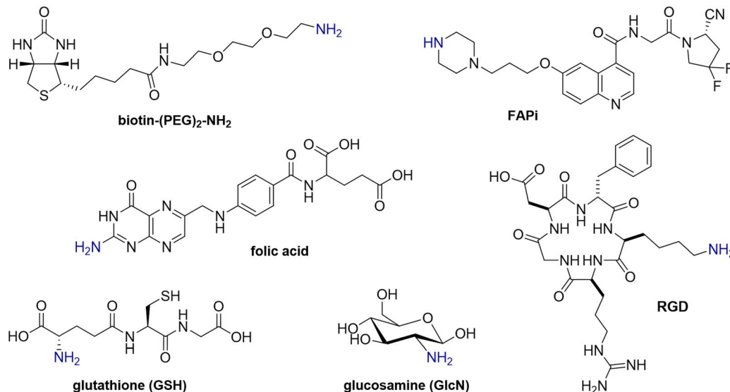
Fig. 2 Structures of R-NH 2 and RR'-NH amines.
