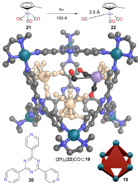
Fig. 6 Representation of the SCXRD structure of (21)_3(22)\text{CO} \subset 19 constructed from ligand 20. Two Mn tricarbonyls 21 and the one Mn dicarbonyl 22 are shown; the third encapsulated Mn tricarbonyl 21 closest to the camera has been omitted for clarity. Disorder, solvent, hydrogen atoms, and counter anions have been omitted for clarity. Colour: C = grey or black, N = blue, O = red, Pd = turquoise, Mn = purple; other atoms of encapsulated complexes = wheat.
