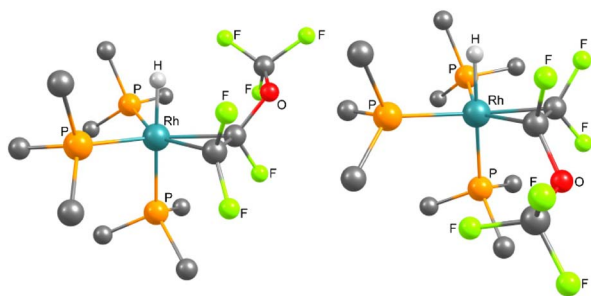
Fig. 1 DFT optimised structures ((B3LYP/cc-pvtz and cc-pvdz, see ESI†) of left: fac - [\text{Rh}(\text{H})(\eta^2\text{-CF}_2=\text{CF}(\text{OCF}_3))(\text{PMe}_3)_3] (2*), and right: (2'*). Hydrogen atoms of the phosphine ligands are omitted for clarity.
