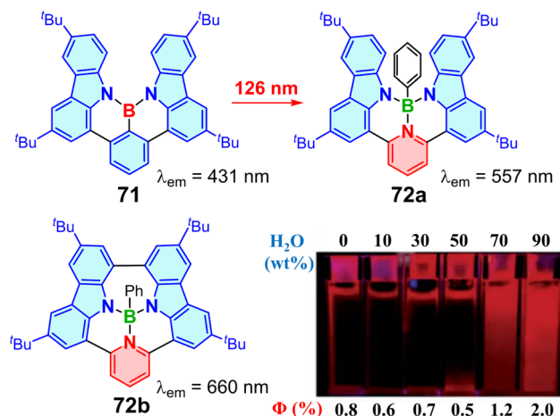
Fig. 22 Tri- and tetra-coordinate boron molecules with NBN fragments and their maximum emission wavelengths in 10^{-5} \text{ M} THF solution. The inset shows the photograph showing the emission intensity increase of 72b with the increasing \text{H}_2\text{O} fraction. Copyright 2022, The Royal Society of Chemistry.
