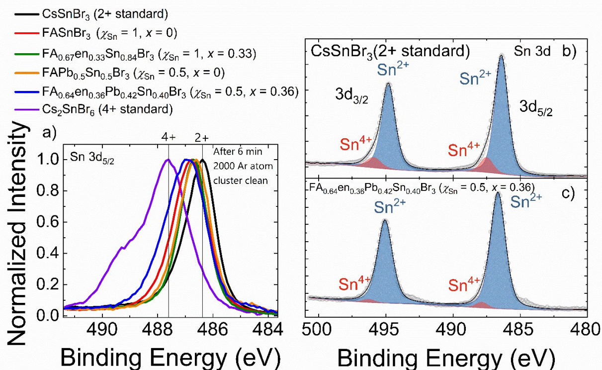
Figure 3. a) Sn 3d 5/2 spectrum of 2 standards (CsSnBr 3 and Cs 2 SnBr 6 ) and selected samples. The samples include a hMHP (FA 0.67 en 0.33 Sn 0.84 Br 3 ( \chi_{\text{Sn}} = 1, x = 0.33 )), a mixed Pb/Sn (FAPb 0.5 Sn 0.5 Br 3 ( \chi_{\text{Sn}} = 0.5, x = 0 )) and both hMHP and Pb/Sn mixed sample (FA 0.64 en 0.36 Pb 0.42 Sn 0.40 Br 3 ( \chi_{\text{Sn}} = 0.5, x = 0.36 )). All samples have a similar FWHM and peak position as the FASnBr 3 . All the samples are mainly Sn 2+ with minor Sn 4+ components. b) Fitted Sn 3d spectra for the 2+ standard showing a small (11%) Sn 4+ contribution compared to sample c) FA 0.64 en 0.36 Pb 0.42 Sn 0.40 Br 3 ( \chi_{\text{Sn}} = 0.5, x = 0.36 ), which showed only 4%.
