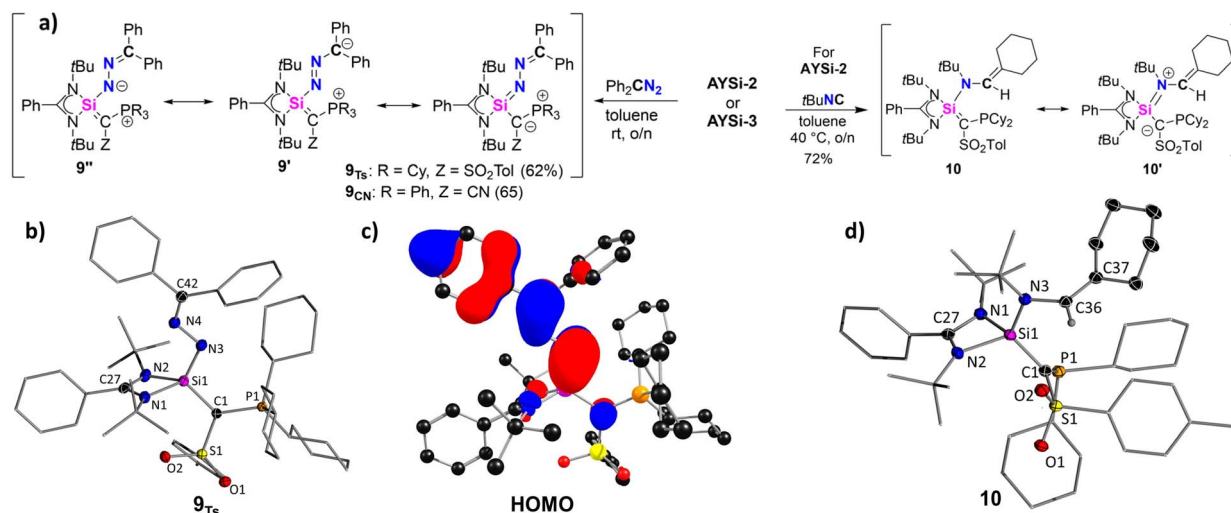
Fig. 8 (a) Reactivity of the AYSi-2 and AYSi-3 with diphenyldiazomethane to obtain 9 Ts and 9 CN and reaction of AYSi-2 with t BuNC yielding 9 . (b) Solid-state structure of 9 Ts . Thermal ellipsoids are shown at the 50% probability level and hydrogen atoms have been omitted for clarity. Important bond lengths [Å] and angles [°]: Si1–C1 1.8437(15), Si1–N3 1.6765(13), N3–N4 1.3848(17), N4–C42 1.2965(19), Si1–N1 1.8370(13), Si1–N2 1.8469(13), C1–Si1–N3 112.66(6), Si1–N3–N4 108.07(9), N3–N4–C42 117.94(12). (c) HOMO of 9 and (d) crystal structure of 10 . Important bond lengths [Å] and angles [°]: Si1–C1 1.8044(13), Si1–N3 1.7230(11), Si1–N1 1.8193(13), Si1–N2 1.8803(11), C1–P1 1.8052(13), N3–C36 1.4502(16), C36–C37 1.3391(19).
