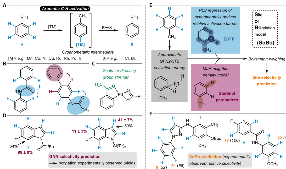
Fig. 9 (A) Schematic reaction mechanism of a C-H activation-mediated C aryl -H substitution reaction. (B) A single directing group favoring two different sites (left) and two different directing groups favoring two different sites (right) during C-H activation. (C) Example of the palladacycle intermediate used by Tomberg et al. to computationally construct a scale for directing group strength. The example directing group is highlighted in green. (D) Borylation site-selectivity predictions made by a three-dimensional GNN model and comparison to the experimental observations. The predicted percentages and respective standard deviations were obtained by applying the model to ten different conformers of the substrate molecule. (E) Schematic representation of the Site of Borylation (SoBo) model architecture and (F) two of its prediction examples in comparison to the experimental observations.
