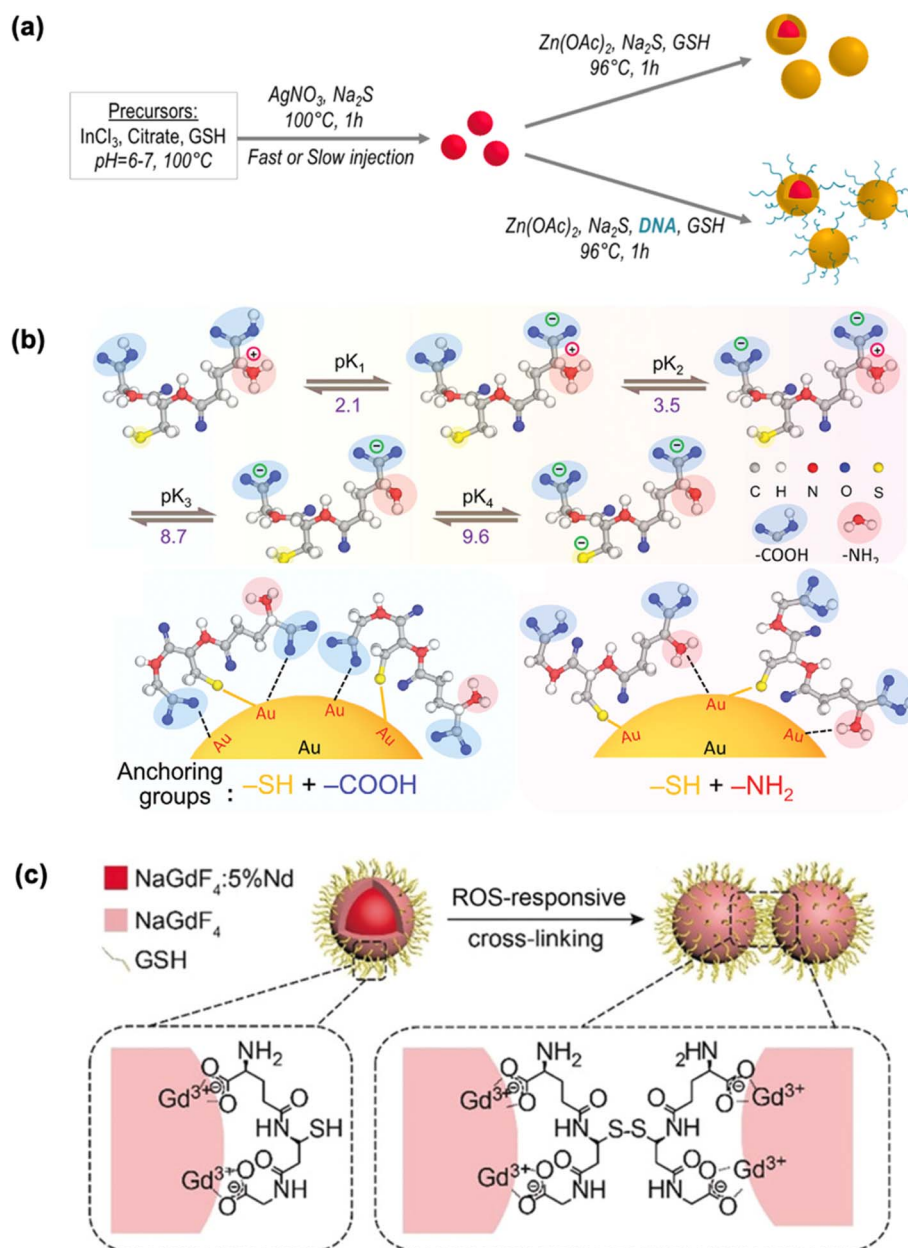
Fig. 2 Synthesis or functionalization of GSH-protected metal nanomaterials enabled by multiple functional groups. (a) Schematic representation of the aqueous synthesis strategy for AIS 2 /ZnS core/shell QDs functionalized with DNA, where GSH is used as a linker for shell growth. Reprinted with permission from ref. 81. Copyright 2020 American Chemical Society. (b) Schematic illustration of step-wise ionization and activation of functional groups of GSH, and the GSH-protected Au NPs synthesized at pH 10.0 (left panel) and pH 2.0 (right panel). Reprinted with permission from ref. 60. Copyright 2021 Wiley. (c) Schematic illustration of bioimaging for acute local epidermal inflammation using the reductive –SH in GSH-protected LNP nanoprobe. The nanoprobe cross-links at the inflamed site in response to ROS and are rapidly excreted from the body. Reprinted with permission from ref. 28. Copyright 2019 Wiley.
