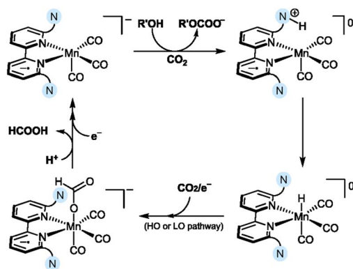
Scheme 10 Proposed reduction mechanism showing the generation of the Mn hydride for amine-substituted Mn complexes, Mn5–Mn7 . 53 The nitrogen atom enclosed in blue denotes a tertiary amine in the secondary coordination sphere.
