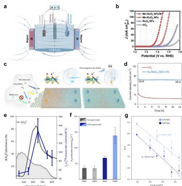
Fig. 11 (a) Schematic illustration of a three-electrode system with applying a magnetic field. (b) LSV curves of Mn–RuO 2 NFs/M, Mn–RuO 2 NFs, RuO 2 NFs, and IrO 2 in 0.5 M H 2 SO 4 . Reproduced with permission from ref. 131 Copyright 2023 Wiley. (c) Illustration of the hydrothermal synthesis of M 1 /MoS 2 SASCs under acidic conditions and the giant magnetic field enhancement of ferromagnetic SASCs for water splitting. (d) Current density versus time curves of Ni 1 /MoS 2 under the magnetic field to compare with that of the IrO 2 in water splitting cells. Reproduced with permission from ref. 132 Copyright 2023 Springer Nature. (e) Wavelength-dependent H 2 production plotted simultaneously with the electric (E) field strength in the hot-spots within the visible range and the weighted absorbance. (f) H 2 generation rate normalized by the total mass of catalyst in both conditions, dark and light, for Au and AuPt supercrystals. (g) Revealing the impact of white-light illumination, the activation energy ( E_a ) for AuPt supercrystal decreased from 33.4 kJ mol −1 to 29.8 kJ mol −1 in the Arrhenius plot analysis. Reproduced with permission from ref. 133 Copyright 2023 Springer Nature.
