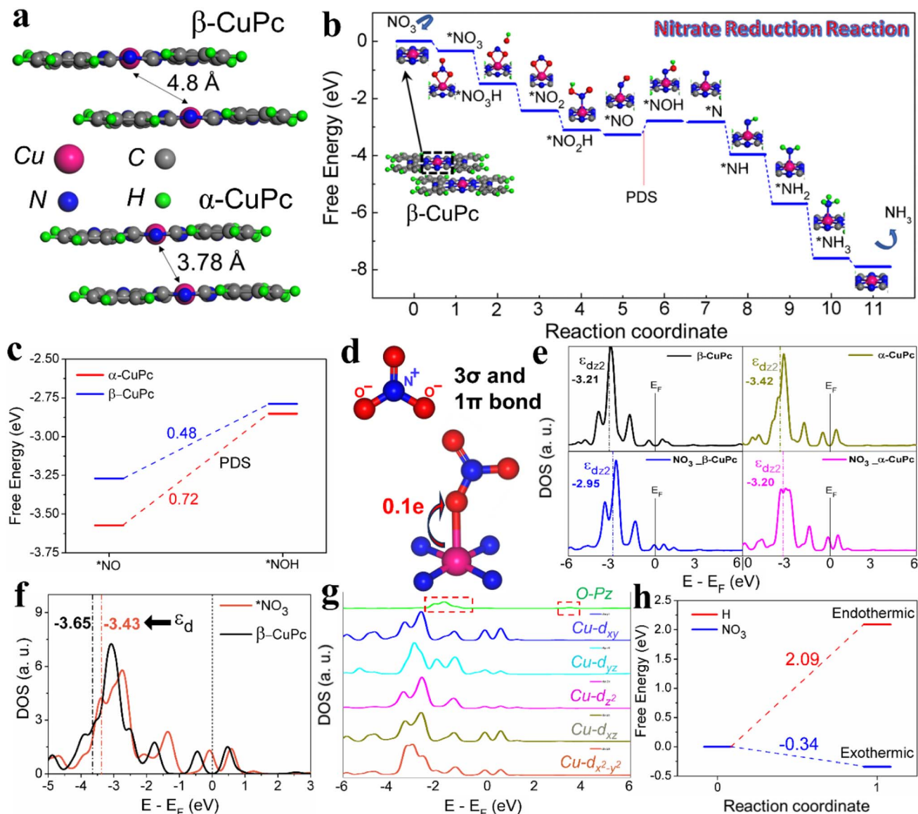
Fig. 4 (a) Model structures of \beta -CuPc and \alpha -CuPc. (b) The free energy profile of the \text{NO}_3 RR on the \beta -CuPc model. (c) The comparison of PDS. (d) The bonding mechanism in the \text{NO}_3 molecule and charge transfer between the Cu site of \beta -CuPc and the O atom of adsorbed \text{NO}_3 . (e) The projected density of states for \beta -CuPc and \alpha -CuPc with and without \text{NO}_3 adsorbed. E_F is defined as the Fermi level at zero on the x-axis. (f) The projected density of states and d band center for the Cu active site in \beta -CuPc and \text{NO}_3 adsorbed \beta -CuPc. (g) The projected density of states for d_{xy} , d_{yz} , d_{xz} , d_{z^2} , and d_{x^2-y^2} orbitals of the Cu active site and the p_z orbital of the O atom in \text{NO}_3 adsorbed \beta -CuPc. (h) The comparison of \text{NO}_3 and hydrogen adsorption on the Cu active site of \beta -CuPc.
