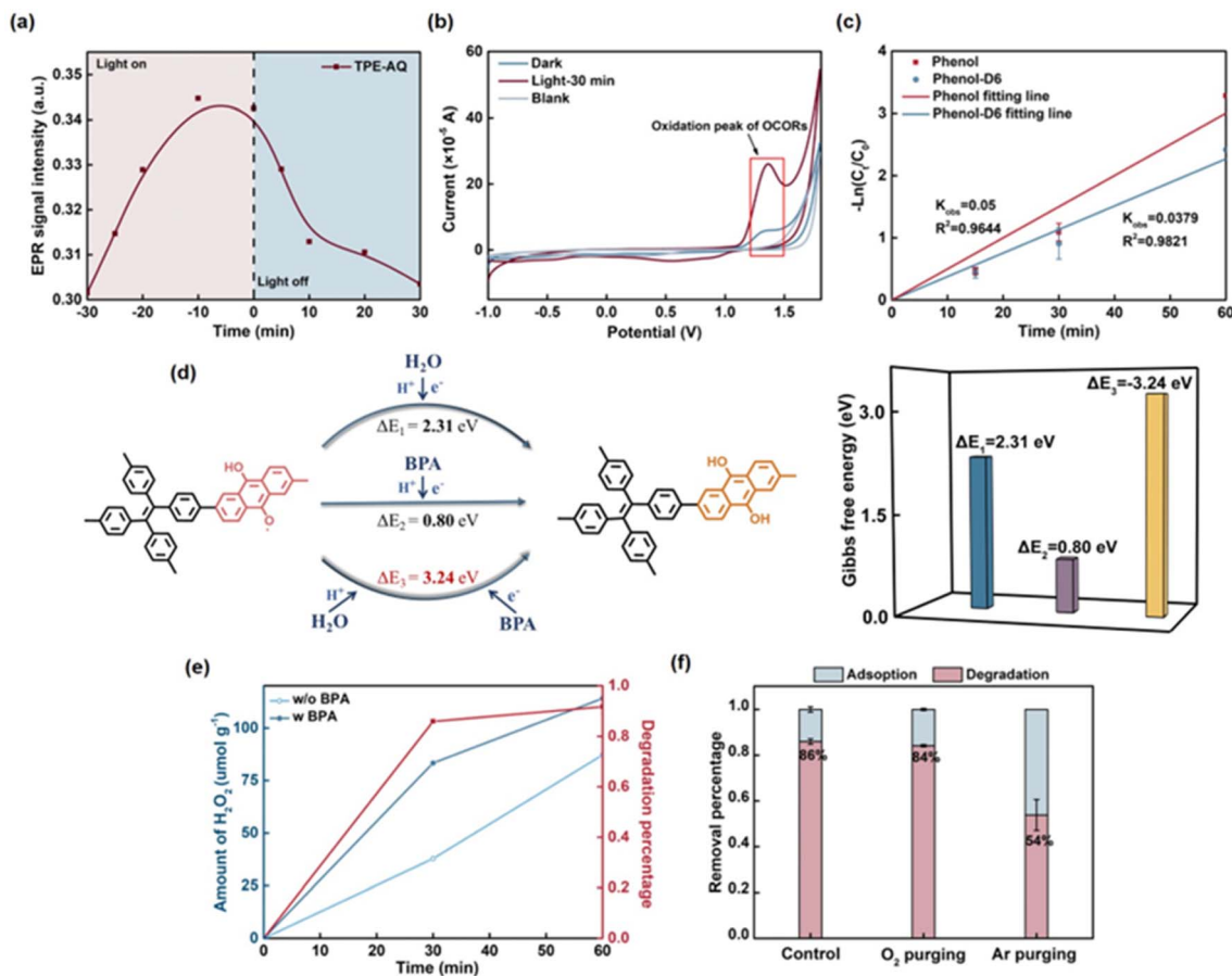
Fig. 7 Quenching and reaction of OCORs. (a) The time-dependent in situ EPR spectra of TPE-AQ in \text{H}_2\text{O} . (b) CV curves of TPE-AQ on glassy carbon electrodes in 0.1 M KCl solution at a sweep rate of 50 \text{ mV s}^{-1} . (c) H/D kinetic isotope effect for phenol degradation in the TPE-AQ system. (d) The Gibbs free energy ( \Delta E ) of OCORs converted to anthrahydroquinone under different conditions. (e) The photocatalytic performance of TPE-AQ for \text{H}_2\text{O}_2 production with or without BPA. (f) Photocatalytic degradation of BPA by TPE-AQ by purging with \text{O}_2 or Ar. Reaction conditions: (c) [\text{phenol}] = [\text{phenol-D6}] = 2 \mu\text{M} , [\text{TPE-AQ}] = 0.05 \text{ g L}^{-1} , and I_0 = 2.0 \text{ mW cm}^{-2} ; (e and f) [\text{BPA}] = 2 \mu\text{M} and [\text{TPE-AQ}] = 0.05 \text{ g L}^{-1} , I_0 = 2.0 \text{ mW cm}^{-2} , and [\text{reaction time}] = 60 \text{ min} (e) and 30 \text{ min} (f).
