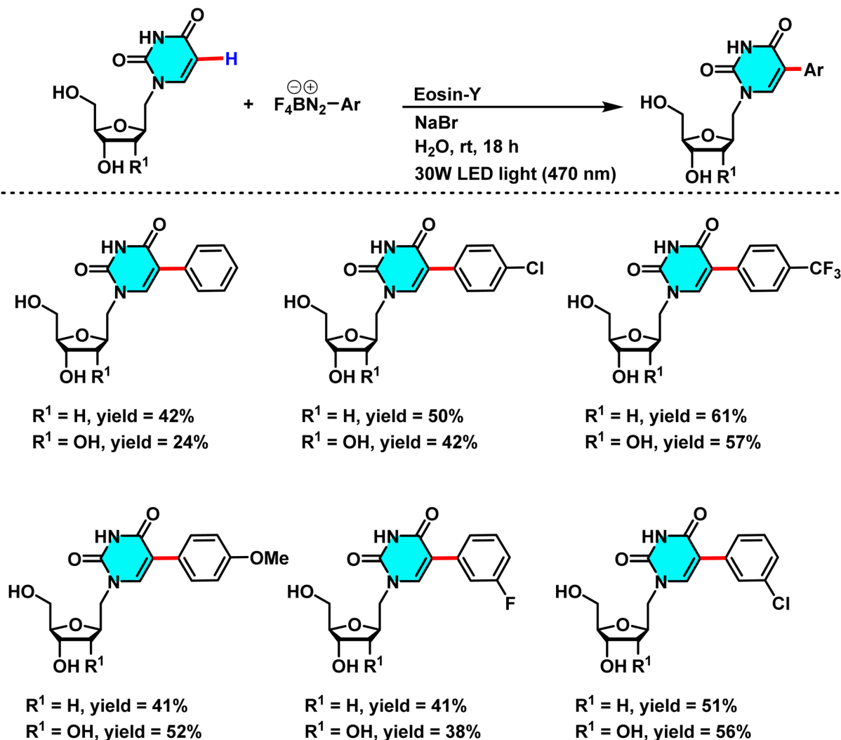
Scheme 94 Photocatalytic C(5)-arylation of uridine and deoxyuridine derivatives using blue LED light (30 W) under metal-free conditions.
