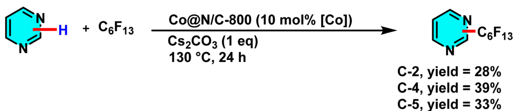
Scheme 40 Direct perfluoroalkylation of pyrimidine using a cobalt-based nanocatalyst.
