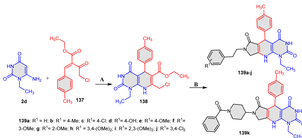
Scheme 47 Formation of pyrrolo[3',4':5,6]pyrido[2,3- d ]pyrimidine-2,4,6(3 H )-triones 139a–k . Reagents and conditions: A; \text{MgSO}_4 , MeOH, 45 °C. B; \text{RNH}_2 , EtOH, Microwave, 120 °C.
