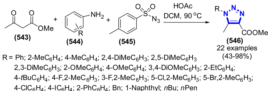
Scheme 144 Preparation of 1,2,3-triazole derivatives catalyzed by acetic acid.
