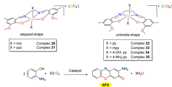
Scheme 12 Complexes 30–35 involving cobalt(III) salts with various heteroaromatic co-ligands, and the oxidation of OAP to APX (ref. 37).
